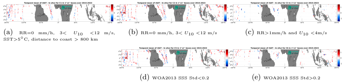
Figure 12: Temporal mean gridded over spatial boxes of size 1^\circ \times 1^\circ of \Delta SSS (SMAP SSS L2 v5.0 (JPL) - TSG (SAMOS)) for 5 different subdatasets corresponding to:RR=0 mm/h, 3 < U_{10} < 12 m/s, SST >5^\circ\text{C} , distance to coast > 800 km (a), RR=0 mm/h, 3 < U_{10} < 12 m/s (b), RR >1 mm/h and U_{10} < 4 m/s (c), WOA2013 SSS Std <0.2 (d), WOA2013 SSS Std >0.2 (e).
