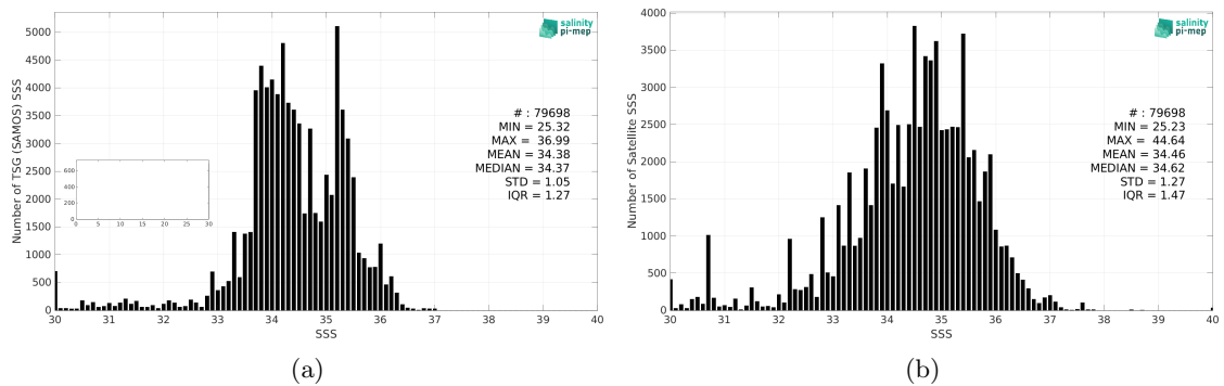
Figure 2: Histograms of SSS from TSG (SAMOS) (a) and SMAP SSS L2 v5.0 (JPL) (b) considering all match-up pairs per bins of 0.1 over the Equatorial Ocean 10N-10S Pi-MEP region and for the full satellite product period.
