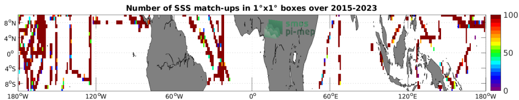
Figure 4: Number of SSS match-ups between TSG (SAMOS) SSS and the SMAP SSS L2 v5.0 (JPL) SSS product for the Equatorial Ocean 10N-10S Pi-MEP region over 1^\circ \times 1^\circ boxes and for the full satellite product period.
