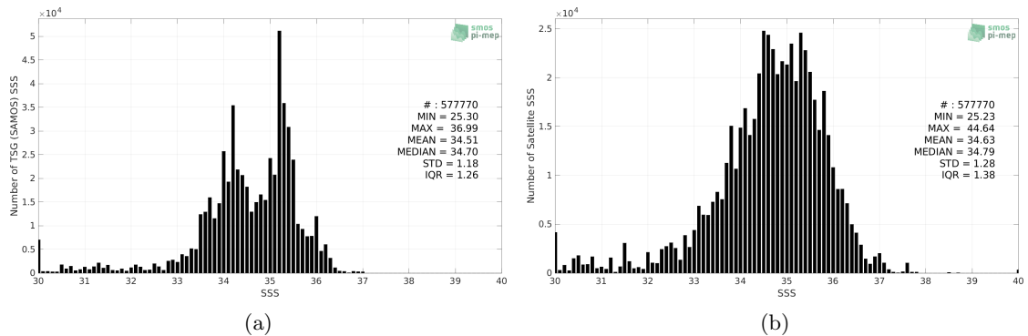
Figure 2: Histograms of SSS from TSG (SAMOS) (a) and SMAP SSS L2 v5.0 (JPL) (b) considering all match-up pairs per bins of 0.1 over the Equatorial Ocean 10N-10S Pi-MEP region and for the full satellite product period.
