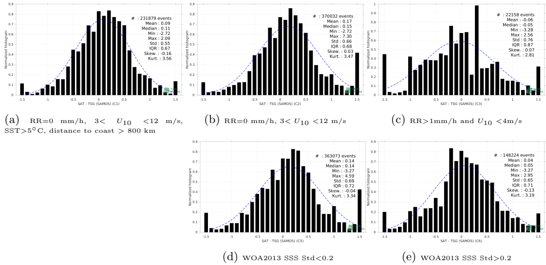
Figure 13: Normalized histogram of \Delta SSS (SMAP SSS L2 v5.0 (JPL) - TSG (SAMOS)) for 5 different subdatasets corresponding to: RR=0 mm/h, 3 < U_{10} < 12 m/s, SST >5^\circ\text{C} , distance to coast > 800 km (a), RR=0 mm/h, 3 < U_{10} < 12 m/s (b), RR >1 mm/h and U_{10} < 4 m/s (c), WOA2013 SSS Std <0.2 (d), WOA2013 SSS Std >0.2 (e).
