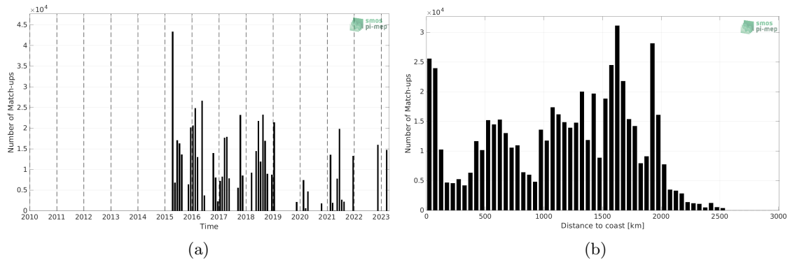
Figure 1: Number of match-ups between TSG (SAMOS) and SMAP SSS L2 v5.0 (JPL) SSS as a function of time (a) and as function of the distance to coast (b) over the Equatorial Ocean 10N-10S Pi-MEP region and for the full satellite product period.
