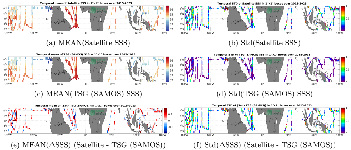
Figure 6: Temporal mean (left) and Std (right) of SSS from SMAP SSS L2 v5.0 (JPL) (top), TSG (SAMOS) (middle), and of \Delta SSS (Satellite - TSG (SAMOS)). Only match-up pairs are used to generate these maps.
