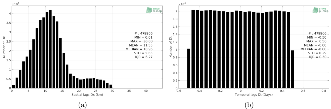
Figure 5: Histograms of the spatial (a) and temporal (b) lags between the time of the TSG (SAMOS) measurements and the date of the corresponding SMAP SSS L2 v5.0 (JPL) SSS product.
