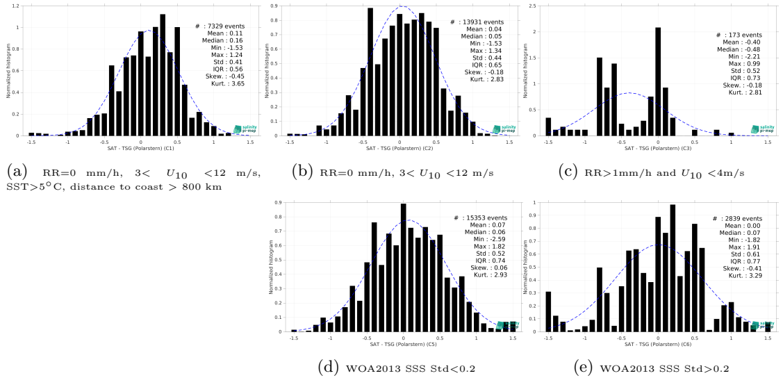
Figure 15: Normalized histogram of \Delta SSS (SMAP SSS L2 v5.0 (JPL) - TSG (Polarstern)) for 5 different subdatasets corresponding to: RR=0 mm/h, 3 < U_{10} < 12 m/s, SST>5°C, distance to coast > 800 km (a), RR=0 mm/h, 3 < U_{10} < 12 m/s (b), RR>1mm/h and U_{10} < 4 m/s (c), WOA2013 SSS Std<0.2 (d), WOA2013 SSS Std>0.2 (e).
