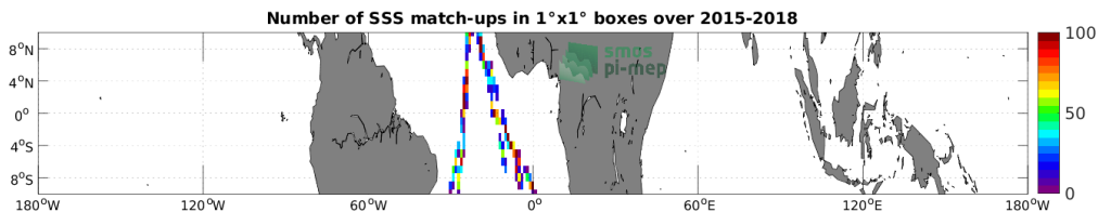
Figure 4: Number of SSS match-ups between TSG (Polarstern) SSS and the SMAP SSS L2 v5.0 (JPL) SSS product for the Equatorial Ocean 10N-10S Pi-MEP region over 1^\circ \times 1^\circ boxes and for the full satellite product period.
