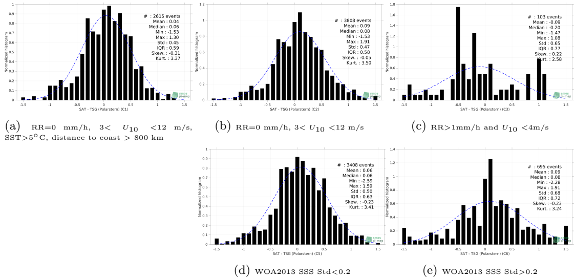
Figure 13: Normalized histogram of \Delta SSS (SMAP SSS L2 v5.0 (JPL) - TSG (Polarstern)) for 5 different subdatasets corresponding to: RR=0 mm/h, 3 < U_{10} < 12 m/s, SST >5^\circ\text{C} , distance to coast > 800 km (a), RR=0 mm/h, 3 < U_{10} < 12 m/s (b), RR >1 mm/h and U_{10} < 4 m/s (c), WOA2013 SSS Std <0.2 (d), WOA2013 SSS Std >0.2 (e).
