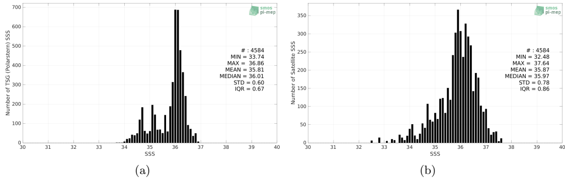
Figure 2: Histograms of SSS from TSG (Polarstern) (a) and SMAP SSS L2 v5.0 (JPL) (b) considering all match-up pairs per bins of 0.1 over the Equatorial Ocean 10N-10S Pi-MEP region and for the full satellite product period.
