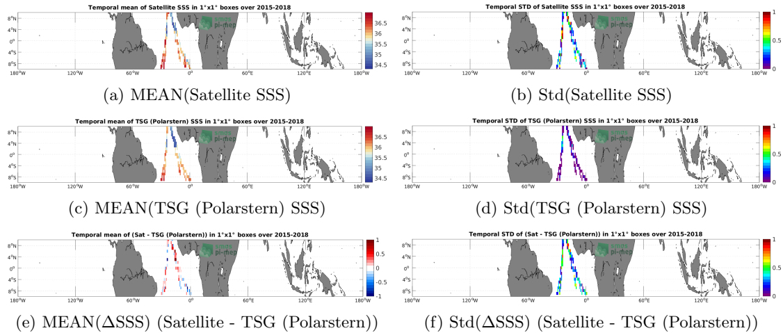
Figure 6: Temporal mean (left) and Std (right) of SSS from SMAP SSS L2 v5.0 (JPL) (top), TSG (Polarstern) (middle), and of \Delta SSS (Satellite - TSG (Polarstern)). Only match-up pairs are used to generate these maps.
