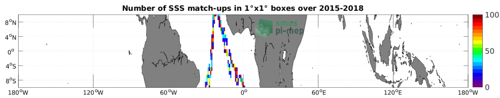
Figure 4: Number of SSS match-ups between TSG (Polarstern) SSS and the SMAP SSS L2 v5.0 (JPL) SSS product for the Equatorial Ocean 10N-10S Pi-MEP region over 1^\circ \times 1^\circ boxes and for the full satellite product period.
