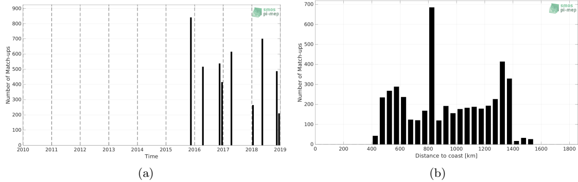
Figure 1: Number of match-ups between TSG (Polarstern) and SMAP SSS L2 v5.0 (JPL) SSS as a function of time (a) and as function of the distance to coast (b) over the Equatorial Ocean 10N-10S Pi-MEP region and for the full satellite product period.
