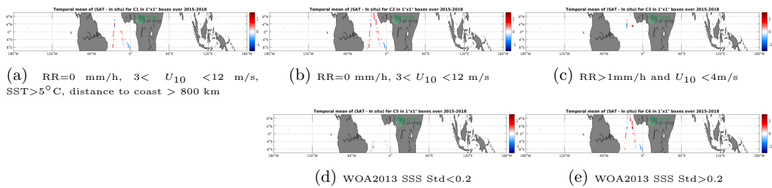
Figure 12: Temporal mean gridded over spatial boxes of size 1°x1° of \Delta SSS (SMAP SSS L2 v5.0 (JPL) - TSG (Polarstern)) for 5 different subdatasets corresponding to: RR=0 mm/h, 3 < U_{10} < 12 m/s, SST > 5°C, distance to coast > 800 km (a), RR=0 mm/h, 3 < U_{10} < 12 m/s (b), RR > 1mm/h and U_{10} < 4m/s (c), WOA2013 SSS Std < 0.2 (d), WOA2013 SSS Std > 0.2 (e).
