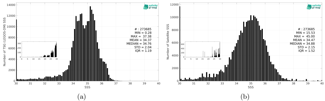
Figure 3: Histograms of SSS from TSG (LEGOS-DM) (a) and SMAP SSS L2 v5.0 (JPL) (b) considering all match-up pairs per bins of 0.1 over the Equatorial Ocean 10N-10S Pi-MEP region and for the full satellite product period.
