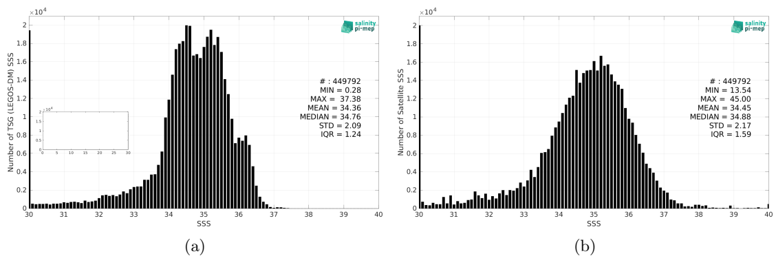
Figure 2: Histograms of SSS from TSG (LEGOS-DM) (a) and SMAP SSS L2 v5.0 (JPL) (b) considering all match-up pairs per bins of 0.1 over the Equatorial Ocean 10N-10S Pi-MEP region and for the full satellite product period.
