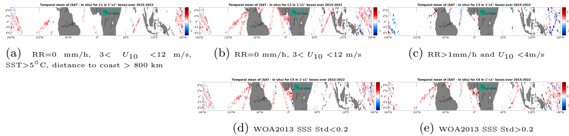
Figure 12: Temporal mean gridded over spatial boxes of size 1^\circ \times 1^\circ of \Delta SSS (SMAP SSS L2 v5.0 (JPL) - TSG (LEGOS-DM)) for 5 different subdatasets corresponding to:RR=0 mm/h, 3 < U_{10} < 12 m/s, SST >5^\circ\text{C} , distance to coast > 800 km (a), RR=0 mm/h, 3 < U_{10} < 12 m/s (b), RR >1 mm/h and U_{10} < 4 m/s (c), WOA2013 SSS Std <0.2 (d), WOA2013 SSS Std >0.2 (e).
