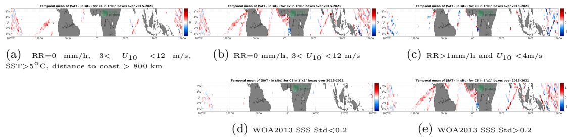
Figure 12: Temporal mean gridded over spatial boxes of size 1^\circ \times 1^\circ of \Delta SSS (SMAP SSS L2 v5.0 (JPL) - TSG (LEGOS-DM)) for 5 different subdatasets corresponding to:RR=0 mm/h, 3 < U_{10} < 12 m/s, SST >5^\circ\text{C} , distance to coast > 800 km (a), RR=0 mm/h, 3 < U_{10} < 12 m/s (b), RR >1 mm/h and U_{10} < 4 m/s (c), WOA2013 SSS Std <0.2 (d), WOA2013 SSS Std >0.2 (e).
