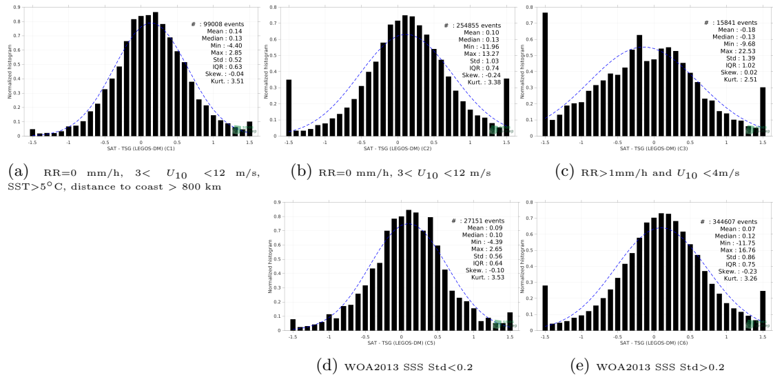
Figure 13: Normalized histogram of \Delta SSS (SMAP SSS L2 v5.0 (JPL) - TSG (LEGOS-DM)) for 5 different subdatasets corresponding to: RR=0 mm/h, 3 < U_{10} < 12 m/s, SST >5^\circ\text{C} , distance to coast > 800 km (a), RR=0 mm/h, 3 < U_{10} < 12 m/s (b), RR >1 mm/h and U_{10} < 4 m/s (c), WOA2013 SSS Std <0.2 (d), WOA2013 SSS Std >0.2 (e).
