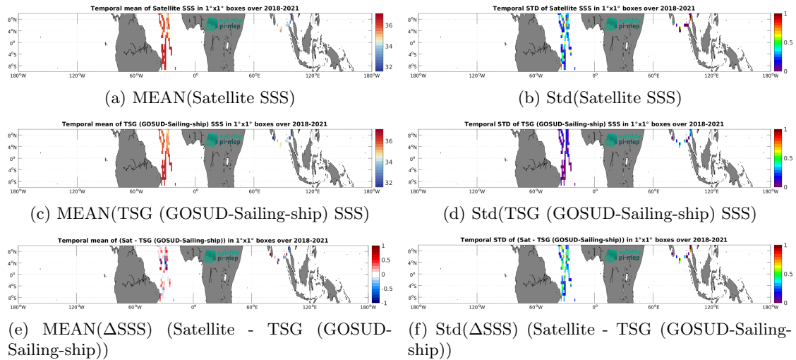
Figure 7: Temporal mean (left) and Std (right) of SSS from SMAP SSS L2 v5.0 (JPL) (top), TSG (GOSUD-Sailing-ship) (middle), and of \Delta SSS (Satellite - TSG (GOSUD-Sailing-ship)). Only match-up pairs are used to generate these maps.
