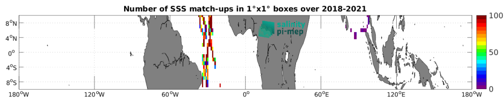
Figure 5: Number of SSS match-ups between TSG (GOSUD-Sailing-ship) SSS and the SMAP SSS L2 v5.0 (JPL) SSS product for the Equatorial Ocean 10N-10S Pi-MEP region over 1^\circ \times 1^\circ boxes and for the full satellite product period.
