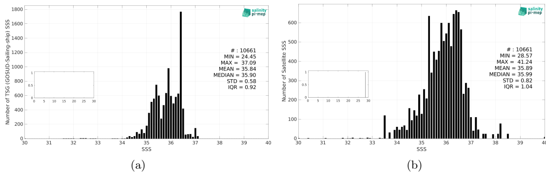
Figure 3: Histograms of SSS from TSG (GOSUD-Sailing-ship) (a) and SMAP SSS L2 v5.0 (JPL) (b) considering all match-up pairs per bins of 0.1 over the Equatorial Ocean 10N-10S Pi-MEP region and for the full satellite product period.
