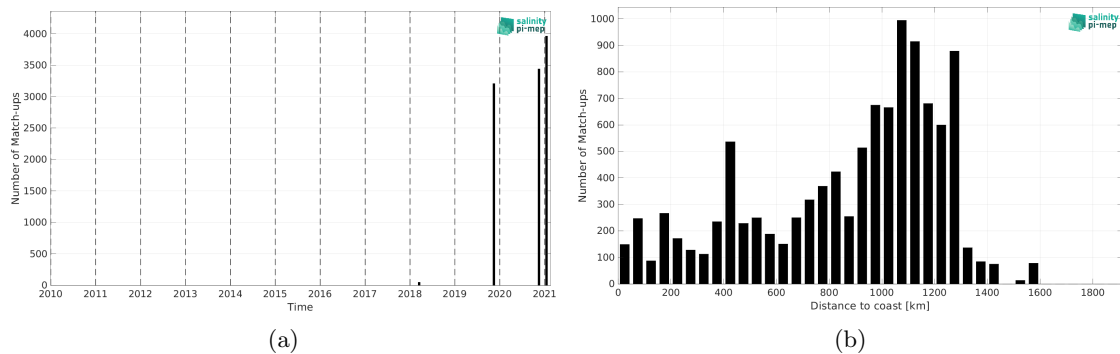
Figure 2: Number of match-ups between TSG (GOSUD-Sailing-ship) and SMAP SSS L2 v5.0 (JPL) SSS as a function of time (a) and as function of the distance to coast (b) over the Equatorial Ocean 10N-10S Pi-MEP region and for the full satellite product period.
