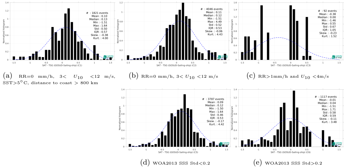
Figure 15: Normalized histogram of \Delta\text{SSS} (SMAP SSS L2 v5.0 (JPL) - TSG (GOSUD-Sailing-ship)) for 5 different subdatasets corresponding to: RR=0 mm/h, 3 < U_{10} < 12 m/s, SST>5°C, distance to coast > 800 km (a), RR=0 mm/h, 3 < U_{10} < 12 m/s (b), RR>1mm/h and U_{10} < 4 m/s (c), WOA2013 SSS Std<0.2 (d), WOA2013 SSS Std>0.2 (e).
