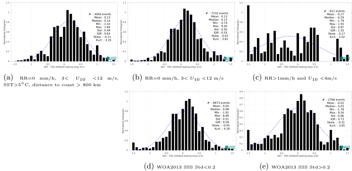
Figure 13: Normalized histogram of \Delta\text{SSS} (SMAP SSS L2 v5.0 (JPL) - TSG (GOSUD-Sailing-ship)) for 5 different subdatasets corresponding to: RR=0 mm/h, 3 < U_{10} < 12 m/s, SST>5°C, distance to coast > 800 km (a), RR=0 mm/h, 3 < U_{10} < 12 m/s (b), RR>1mm/h and U_{10} < 4 m/s (c), WOA2013 SSS Std<0.2 (d), WOA2013 SSS Std>0.2 (e).
