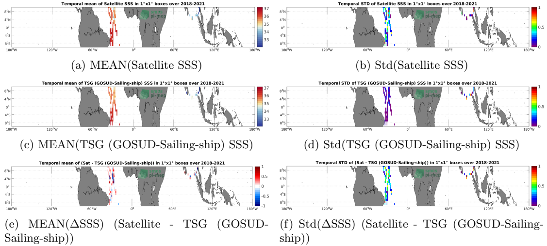
Figure 6: Temporal mean (left) and Std (right) of SSS from SMAP SSS L2 v5.0 (JPL) (top), TSG (GOSUD-Sailing-ship) (middle), and of \Delta SSS (Satellite - TSG (GOSUD-Sailing-ship)). Only match-up pairs are used to generate these maps.
