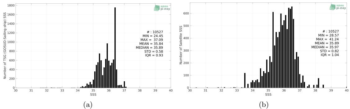
Figure 2: Histograms of SSS from TSG (GOSUD-Sailing-ship) (a) and SMAP SSS L2 v5.0 (JPL) (b) considering all match-up pairs per bins of 0.1 over the Equatorial Ocean 10N-10S Pi-MEP region and for the full satellite product period.
