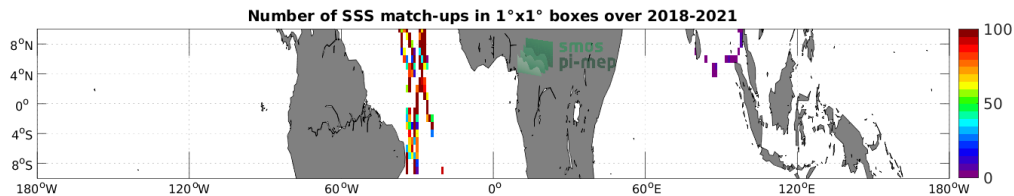
Figure 4: Number of SSS match-ups between TSG (GOSUD-Sailing-ship) SSS and the SMAP SSS L2 v5.0 (JPL) SSS product for the Equatorial Ocean 10N-10S Pi-MEP region over 1^\circ \times 1^\circ boxes and for the full satellite product period.
