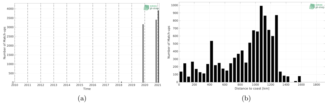
Figure 1: Number of match-ups between TSG (GOSUD-Sailing-ship) and SMAP SSS L2 v5.0 (JPL) SSS as a function of time (a) and as function of the distance to coast (b) over the Equatorial Ocean 10N-10S Pi-MEP region and for the full satellite product period.
