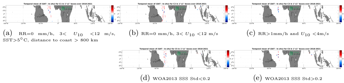
Figure 12: Temporal mean gridded over spatial boxes of size 1^\circ \times 1^\circ of \Delta SSS (SMAP SSS L2 v5.0 (JPL) - TSG (GOSUD-Sailing-ship)) for 5 different subdatasets corresponding to: RR=0 mm/h, 3 < U_{10} < 12 m/s, SST>5°C, distance to coast > 800 km (a), RR=0 mm/h, 3 < U_{10} < 12 m/s (b), RR>1mm/h and U_{10} < 4 m/s (c), WOA2013 SSS Std<0.2 (d), WOA2013 SSS Std>0.2 (e).
