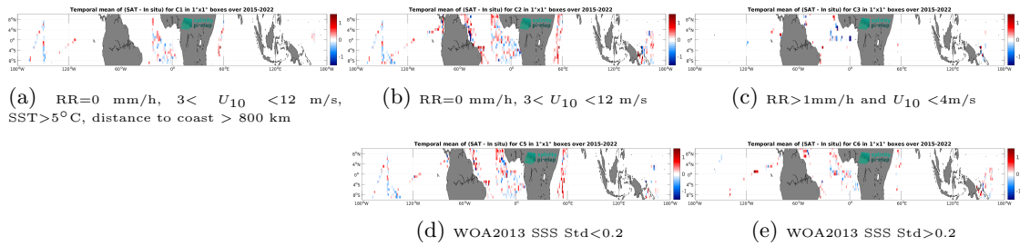
Figure 14: Temporal mean gridded over spatial boxes of size 1^\circ \times 1^\circ of \Delta SSS (SMAP SSS L2 v5.0 (JPL) - TSG (GOSUD-Research-vessel)) for 5 different subdatasets corresponding to: RR=0 mm/h, 3 < U_{10} < 12 m/s, SST>5°C, distance to coast > 800 km (a), RR=0 mm/h, 3 < U_{10} < 12 m/s (b), RR>1mm/h and U_{10} < 4 m/s (c), WOA2013 SSS Std<0.2 (d), WOA2013 SSS Std>0.2 (e).
