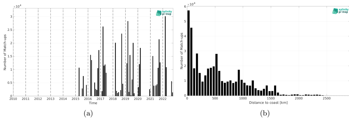
Figure 2: Number of match-ups between TSG (GOSUD-Research-vessel) and SMAP SSS L2 v5.0 (JPL) SSS as a function of time (a) and as function of the distance to coast (b) over the Equatorial Ocean 10N-10S Pi-MEP region and for the full satellite product period.
