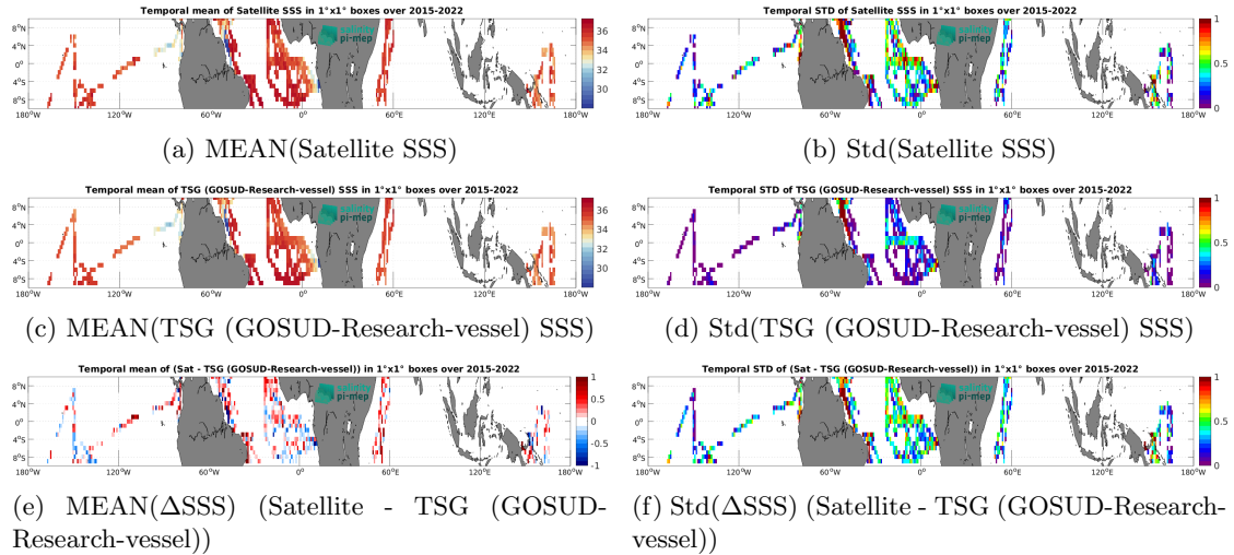
Figure 7: Temporal mean (left) and Std (right) of SSS from SMAP SSS L2 v5.0 (JPL) (top), TSG (GOSUD-Research-vessel) (middle), and of \Delta SSS (Satellite - TSG (GOSUD-Research-vessel)). Only match-up pairs are used to generate these maps.
