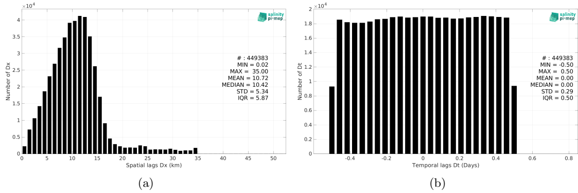
Figure 6: Histograms of the spatial (a) and temporal (b) lags between the location/time of the TSG (GOSUD-Research-vessel) measurement and the date of the corresponding SMAP SSS L2 v5.0 (JPL) SSS pixel.
