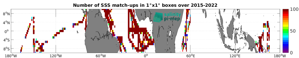
Figure 5: Number of SSS match-ups between TSG (GOSUD-Research-vessel) SSS and the SMAP SSS L2 v5.0 (JPL) SSS product for the Equatorial Ocean 10N-10S Pi-MEP region over 1^\circ \times 1^\circ boxes and for the full satellite product period.
