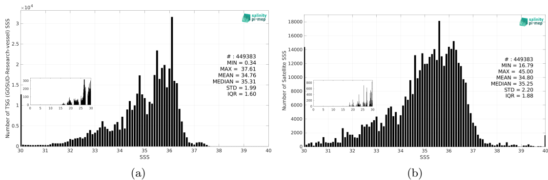
Figure 3: Histograms of SSS from TSG (GOSUD-Research-vessel) (a) and SMAP SSS L2 v5.0 (JPL) (b) considering all match-up pairs per bins of 0.1 over the Equatorial Ocean 10N-10S Pi-MEP region and for the full satellite product period.
