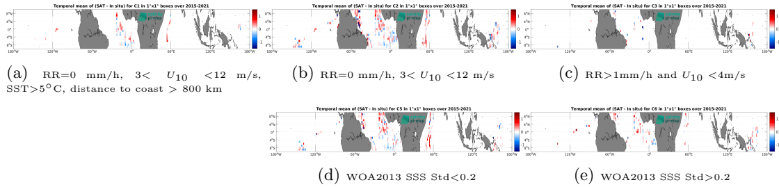
Figure 14: Temporal mean gridded over spatial boxes of size 1^\circ \times 1^\circ of \Delta SSS (SMAP SSS L2 v5.0 (JPL) - TSG (GOSUD-Research-vessel)) for 5 different subdatasets corresponding to: RR=0 mm/h, 3 < U_{10} < 12 m/s, SST>5°C, distance to coast > 800 km (a), RR=0 mm/h, 3 < U_{10} < 12 m/s (b), RR>1mm/h and U_{10} < 4 m/s (c), WOA2013 SSS Std<0.2 (d), WOA2013 SSS Std>0.2 (e).
