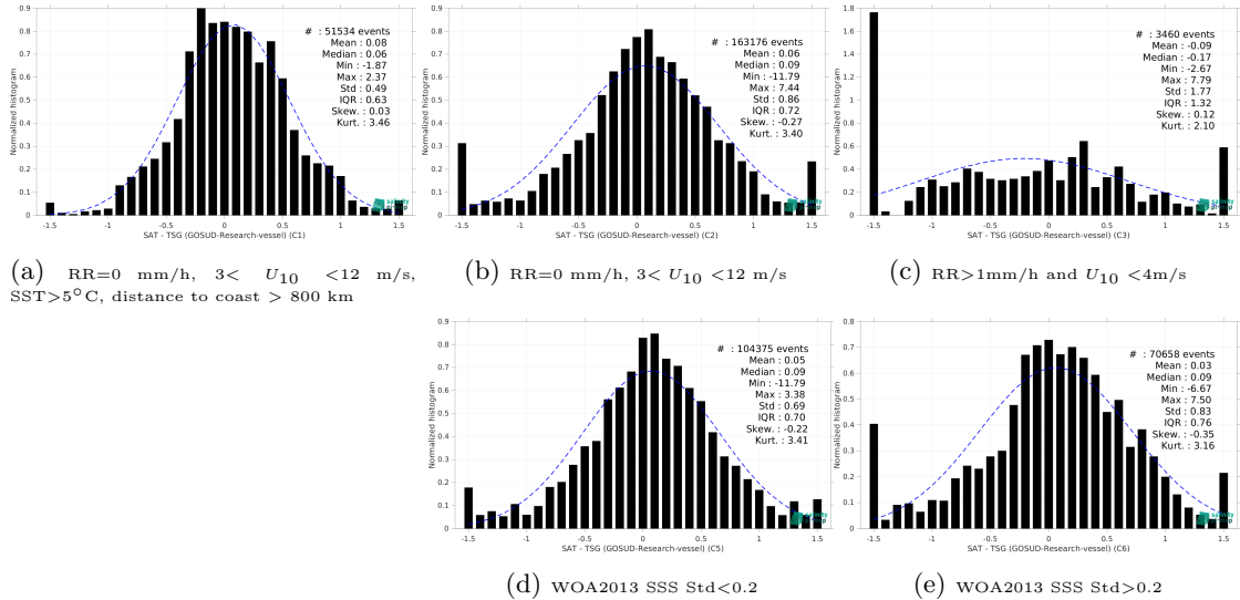
Figure 15: Normalized histogram of \Delta SSS (SMAP SSS L2 v5.0 (JPL) - TSG (GOSUD-Research-vessel)) for 5 different subdatasets corresponding to: RR=0 mm/h, 3 < U_{10} < 12 m/s, SST>5°C, distance to coast > 800 km (a), RR=0 mm/h, 3 < U_{10} < 12 m/s (b), RR>1mm/h and U_{10} < 4 m/s (c), WOA2013 SSS Std<0.2 (d), WOA2013 SSS Std>0.2 (e).
