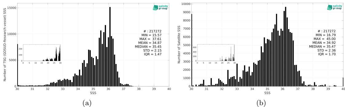
Figure 3: Histograms of SSS from TSG (GOSUD-Research-vessel) (a) and SMAP SSS L2 v5.0 (JPL) (b) considering all match-up pairs per bins of 0.1 over the Equatorial Ocean 10N-10S Pi-MEP region and for the full satellite product period.
