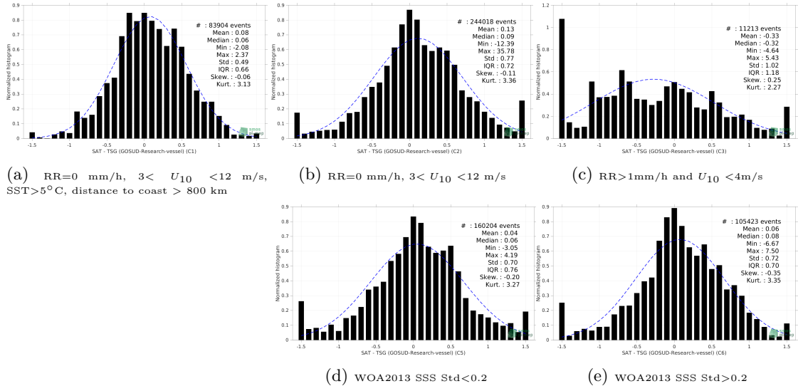
Figure 13: Normalized histogram of \Delta SSS (SMAP SSS L2 v5.0 (JPL) - TSG (GOSUD-Research-vessel)) for 5 different subdatasets corresponding to: RR=0 mm/h, 3 < U_{10} < 12 m/s, SST>5°C, distance to coast > 800 km (a), RR=0 mm/h, 3 < U_{10} < 12 m/s (b), RR>1mm/h and U_{10} < 4 m/s (c), WOA2013 SSS Std<0.2 (d), WOA2013 SSS Std>0.2 (e).
