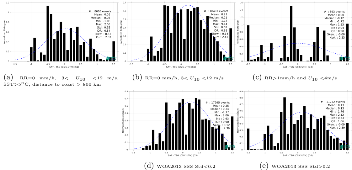
Figure 15: Normalized histogram of \Delta\text{SSS} (SMAP SSS L2 v5.0 (JPL) - TSG (CSIC-UTM)) for 5 different subdatasets corresponding to: RR=0 mm/h, 3 < U_{10} < 12 m/s, SST>5°C, distance to coast > 800 km (a), RR=0 mm/h, 3 < U_{10} < 12 m/s (b), RR>1mm/h and U_{10} < 4 m/s (c), WOA2013 SSS Std<0.2 (d), WOA2013 SSS Std>0.2 (e).
