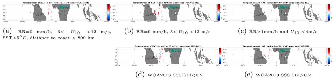
Figure 12: Temporal mean gridded over spatial boxes of size 1^\circ \times 1^\circ of \Delta SSS (SMAP SSS L2 v5.0 (JPL) - TSG (CSIC-UTM)) for 5 different subdatasets corresponding to:RR=0 mm/h, 3 < U_{10} < 12 m/s, SST > 5^\circ C , distance to coast > 800 km (a), RR=0 mm/h, 3 < U_{10} < 12 m/s (b), RR>1mm/h and U_{10} < 4 m/s (c), WOA2013 SSS Std<0.2 (d), WOA2013 SSS Std>0.2 (e).
