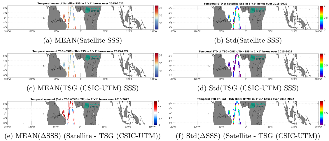
Figure 6: Temporal mean (left) and Std (right) of SSS from SMAP SSS L2 v5.0 (JPL) (top), TSG (CSIC-UTM) (middle), and of \Delta SSS (Satellite - TSG (CSIC-UTM)). Only match-up pairs are used to generate these maps.
