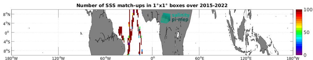
Figure 4: Number of SSS match-ups between TSG (CSIC-UTM) SSS and the SMAP SSS L2 v5.0 (JPL) SSS product for the Equatorial Ocean 10N-10S Pi-MEP region over 1^\circ \times 1^\circ boxes and for the full satellite product period.
