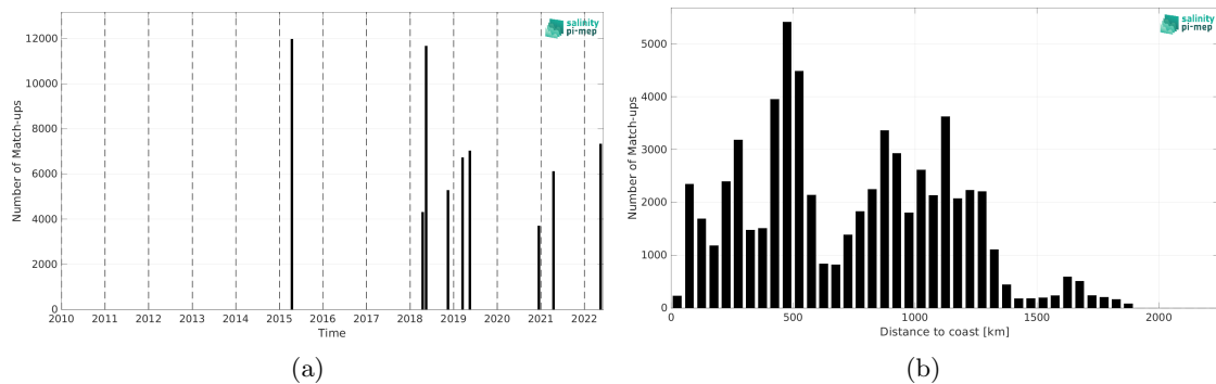
Figure 1: Number of match-ups between TSG (CSIC-UTM) and SMAP SSS L2 v5.0 (JPL) SSS as a function of time (a) and as function of the distance to coast (b) over the Equatorial Ocean 10N-10S Pi-MEP region and for the full satellite product period.
