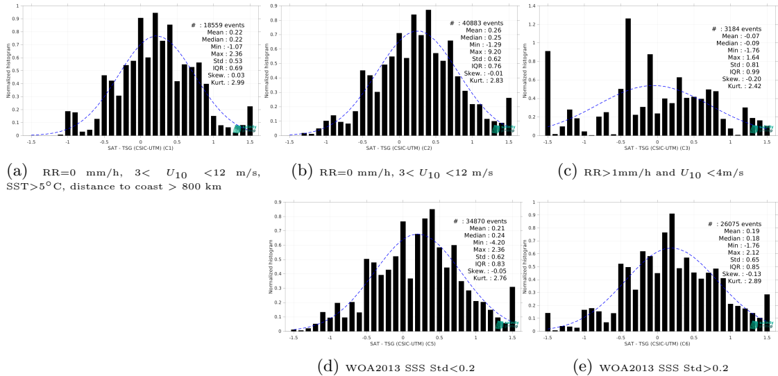
Figure 13: Normalized histogram of \Delta SSS (SMAP SSS L2 v5.0 (JPL) - TSG (CSIC-UTM)) for 5 different subdatasets corresponding to: RR=0 mm/h, 3 < U_{10} < 12 m/s, SST > 5^\circ C , distance to coast > 800 km (a), RR=0 mm/h, 3 < U_{10} < 12 m/s (b), RR>1mm/h and U_{10} < 4 m/s (c), WOA2013 SSS Std<0.2 (d), WOA2013 SSS Std>0.2 (e).
