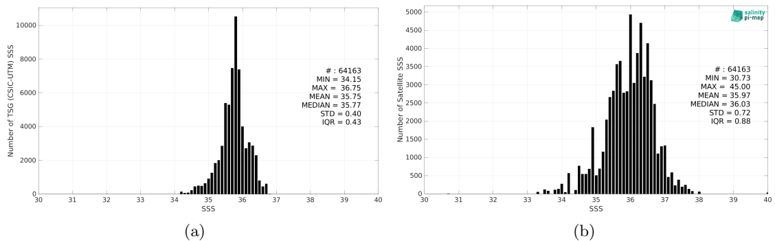
Figure 2: Histograms of SSS from TSG (CSIC-UTM) (a) and SMAP SSS L2 v5.0 (JPL) (b) considering all match-up pairs per bins of 0.1 over the Equatorial Ocean 10N-10S Pi-MEP region and for the full satellite product period.
