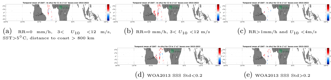
Figure 12: Temporal mean gridded over spatial boxes of size 1^\circ \times 1^\circ of \Delta SSS (SMAP SSS L2 v5.0 (JPL) - TSG (CSIC-UTM)) for 5 different subdatasets corresponding to:RR=0 mm/h, 3 < U_{10} < 12 m/s, SST > 5^\circ C , distance to coast > 800 km (a), RR=0 mm/h, 3 < U_{10} < 12 m/s (b), RR>1mm/h and U_{10} < 4 m/s (c), WOA2013 SSS Std<0.2 (d), WOA2013 SSS Std>0.2 (e).
