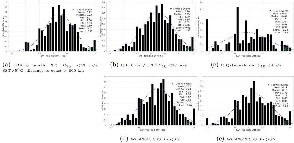
Figure 13: Normalized histogram of \Delta SSS (SMAP SSS L2 v5.0 (JPL) - TSG (CSIC-UTM)) for 5 different subdatasets corresponding to: RR=0 mm/h, 3 < U_{10} < 12 m/s, SST > 5^\circ C , distance to coast > 800 km (a), RR=0 mm/h, 3 < U_{10} < 12 m/s (b), RR>1mm/h and U_{10} < 4 m/s (c), WOA2013 SSS Std<0.2 (d), WOA2013 SSS Std>0.2 (e).
