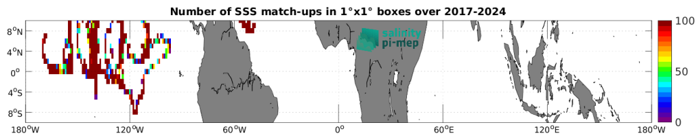
Figure 5: Number of SSS match-ups between Saildrone SSS and the SMAP SSS L2 v5.0 (JPL) SSS product for the Equatorial Ocean 10N-10S Pi-MEP region over 1^\circ \times 1^\circ boxes and for the full satellite product period.
