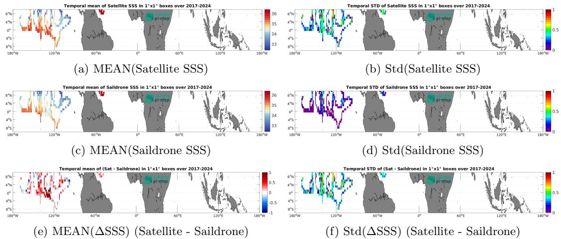
Figure 7: Temporal mean (left) and Std (right) of SSS from SMAP SSS L2 v5.0 (JPL) (top), Saildrone (middle), and of \Delta SSS (Satellite - Saildrone). Only match-up pairs are used to generate these maps.
