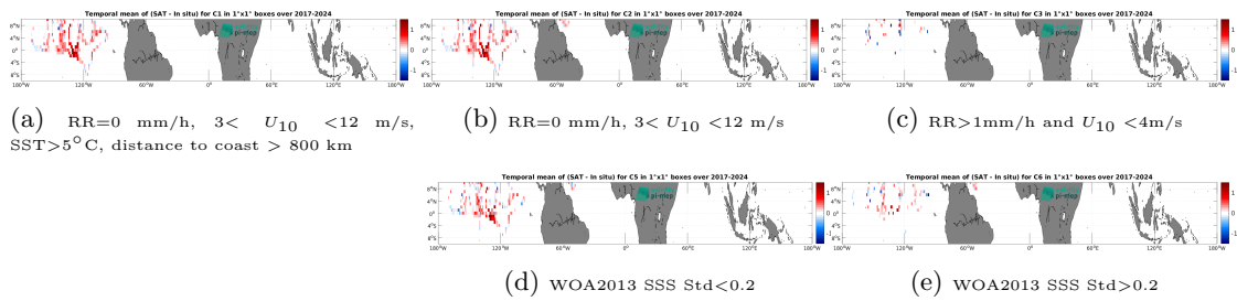
Figure 14: Temporal mean gridded over spatial boxes of size 1^\circ \times 1^\circ of \Delta SSS (SMAP SSS L2 v5.0 (JPL) - Saildrone) for 5 different subdatasets corresponding to:RR=0 mm/h, 3 < U_{10} < 12 m/s, SST>5°C, distance to coast > 800 km (a), RR=0 mm/h, 3 < U_{10} < 12 m/s (b), RR>1mm/h and U_{10} < 4 m/s (c), WOA2013 SSS Std<0.2 (d), WOA2013 SSS Std>0.2 (e).
