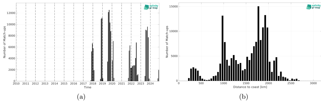
Figure 2: Number of match-ups between Saildrone and SMAP SSS L2 v5.0 (JPL) SSS as a function of time (a) and as function of the distance to coast (b) over the Equatorial Ocean 10N-10S Pi-MEP region and for the full satellite product period.
