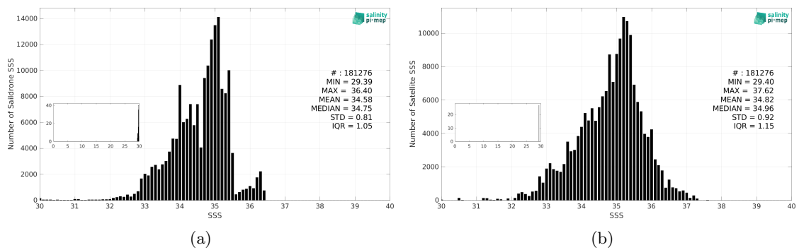
Figure 3: Histograms of SSS from Saildrone (a) and SMAP SSS L2 v5.0 (JPL) (b) considering all match-up pairs per bins of 0.1 over the Equatorial Ocean 10N-10S Pi-MEP region and for the full satellite product period.
