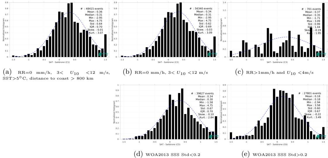
Figure 15: Normalized histogram of \Delta SSS (SMAP SSS L2 v5.0 (JPL) - Saildrone) for 5 different subdatasets corresponding to: RR=0 mm/h, 3 < U_{10} < 12 m/s, SST>5°C, distance to coast > 800 km (a), RR=0 mm/h, 3 < U_{10} < 12 m/s (b), RR>1mm/h and U_{10} < 4 m/s (c), WOA2013 SSS Std<0.2 (d), WOA2013 SSS Std>0.2 (e).
