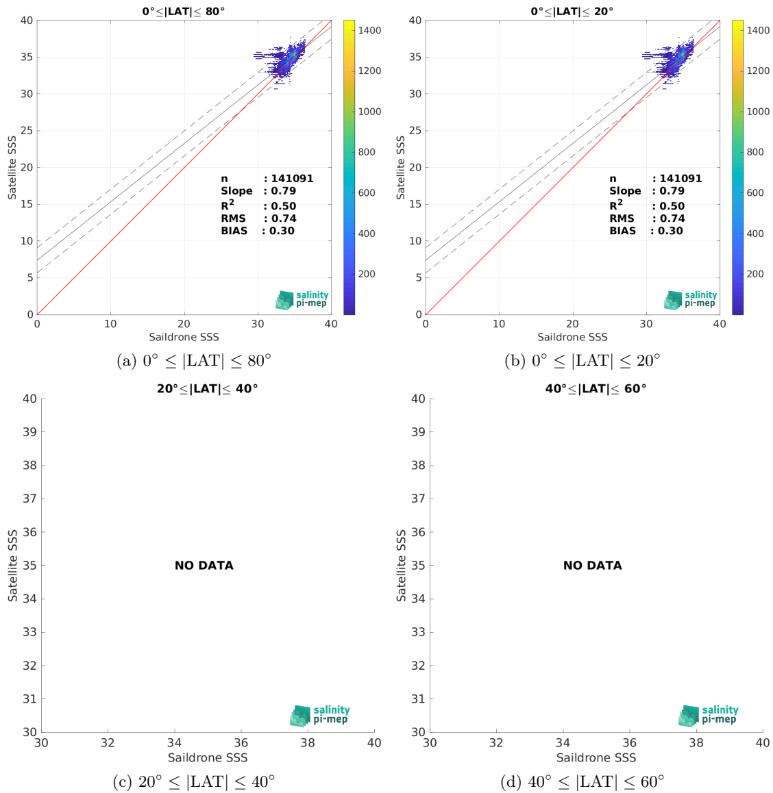
Figure 9: Contour maps of the concentration of SMAP SSS L2 v5.0 (JPL) SSS (y-axis) versus Sairdrone SSS (x-axis) at match-up pairs for different latitude bands. For each plot, the red line shows x=y . The black thin and dashed lines indicate a linear fit through the data cloud and the \pm 95\% confidence levels, respectively. The number match-up pairs n , the slope and R^2 coefficient of the linear fit, the root mean square (RMS) and the mean bias between satellite and in situ data are indicated for each latitude band in each plots.
