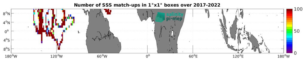
Figure 4: Number of SSS match-ups between Saildrone SSS and the SMAP SSS L2 v5.0 (JPL) SSS product for the Equatorial Ocean 10N-10S Pi-MEP region over 1^\circ \times 1^\circ boxes and for the full satellite product period.
