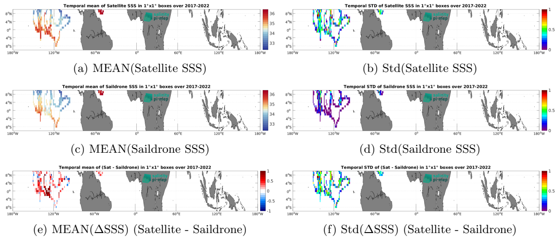
Figure 6: Temporal mean (left) and Std (right) of SSS from SMAP SSS L2 v5.0 (JPL) (top), Saildrone (middle), and of \Delta SSS (Satellite - Saildrone). Only match-up pairs are used to generate these maps.
