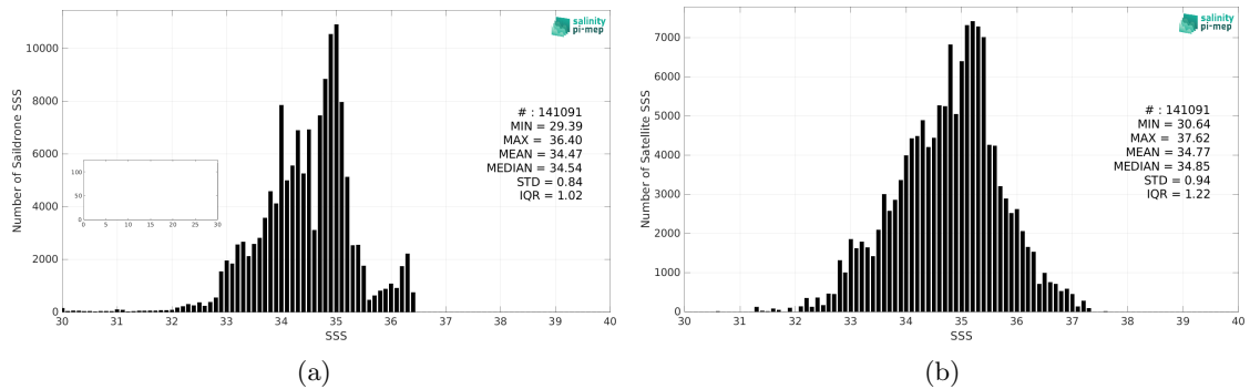
Figure 2: Histograms of SSS from Saildrone (a) and SMAP SSS L2 v5.0 (JPL) (b) considering all match-up pairs per bins of 0.1 over the Equatorial Ocean 10N-10S Pi-MEP region and for the full satellite product period.
