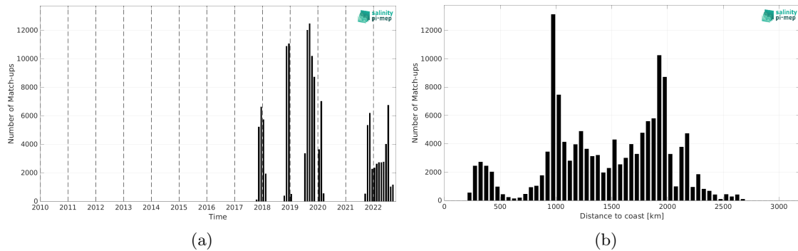
Figure 1: Number of match-ups between Saildrone and SMAP SSS L2 v5.0 (JPL) SSS as a function of time (a) and as function of the distance to coast (b) over the Equatorial Ocean 10N-10S Pi-MEP region and for the full satellite product period.
