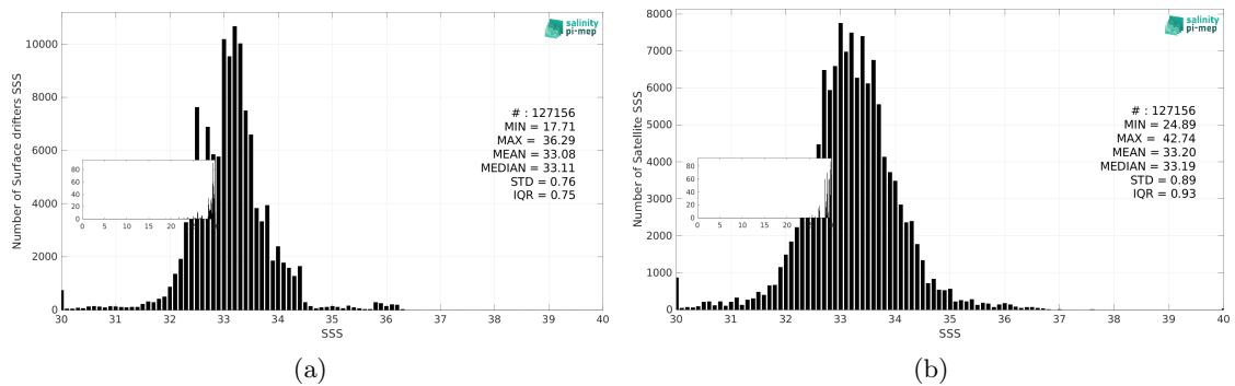
Figure 3: Histograms of SSS from Surface drifters (a) and SMAP SSS L2 v5.0 (JPL) (b) considering all match-up pairs per bins of 0.1 over the Equatorial Ocean 10N-10S Pi-MEP region and for the full satellite product period.
