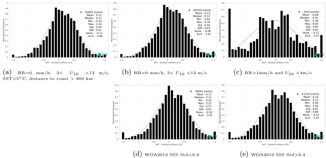
Figure 14: Normalized histogram of \Delta SSS (SMAP SSS L2 v5.0 (JPL) - Surface drifters) for 5 different subdatasets corresponding to: RR=0 mm/h, 3 < U_{10} < 12 m/s, SST >5^\circ C , distance to coast > 800 km (a), RR=0 mm/h, 3 < U_{10} < 12 m/s (b), RR >1 mm/h and U_{10} < 4 m/s (c), WOA2013 SSS Std <0.2 (d), WOA2013 SSS Std >0.2 (e).
