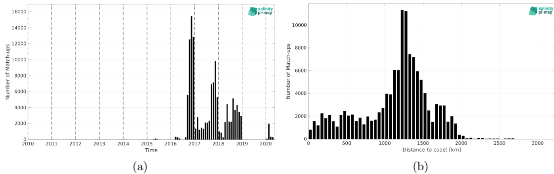
Figure 2: Number of match-ups between Surface drifters and SMAP SSS L2 v5.0 (JPL) SSS as a function of time (a) and as function of the distance to coast (b) over the Equatorial Ocean 10N-10S Pi-MEP region and for the full satellite product period.
