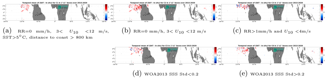
Figure 11: Temporal mean gridded over spatial boxes of size 1^\circ \times 1^\circ of \Delta SSS (SMAP SSS L2 v5.0 (JPL) - Surface drifters) for 5 different subdatasets corresponding to:RR=0 mm/h, 3 < U_{10} < 12 m/s, SST>5°C, distance to coast > 800 km (a), RR=0 mm/h, 3 < U_{10} < 12 m/s (b), RR>1mm/h and U_{10} < 4 m/s (c), WOA2013 SSS Std<0.2 (d), WOA2013 SSS Std>0.2 (e).
