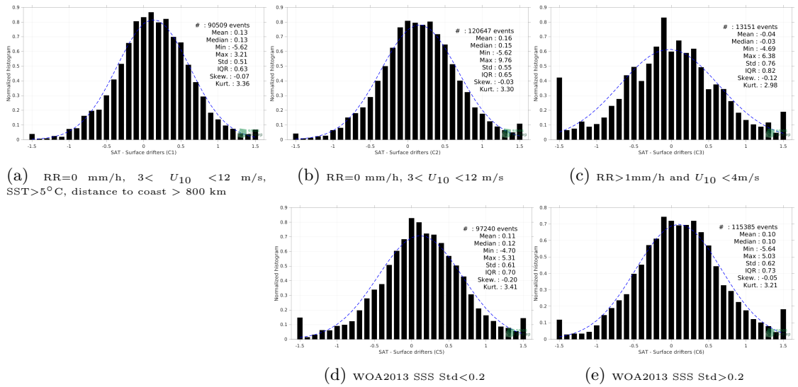
Figure 12: Normalized histogram of \Delta SSS (SMAP SSS L2 v5.0 (JPL) - Surface drifters) for 5 different subdatasets corresponding to: RR=0 mm/h, 3 < U_{10} < 12 m/s, SST >5^\circ\text{C} , distance to coast > 800 km (a), RR=0 mm/h, 3 < U_{10} < 12 m/s (b), RR >1 mm/h and U_{10} < 4 m/s (c), WOA2013 SSS Std <0.2 (d), WOA2013 SSS Std >0.2 (e).
