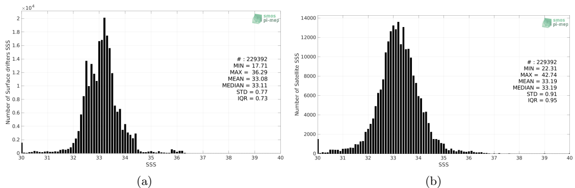
Figure 2: Histograms of SSS from Surface drifters (a) and SMAP SSS L2 v5.0 (JPL) (b) considering all match-up pairs per bins of 0.1 over the Equatorial Ocean 10N-10S Pi-MEP region and for the full satellite product period.
