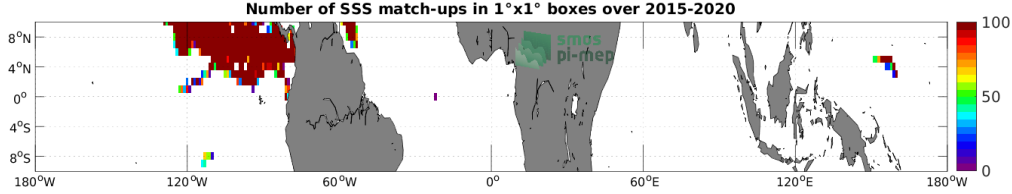
Figure 3: Number of SSS match-ups between Surface drifters SSS and the SMAP SSS L2 v5.0 (JPL) SSS product for the Equatorial Ocean 10N-10S Pi-MEP region over 1^\circ \times 1^\circ boxes and for the full satellite product period.
