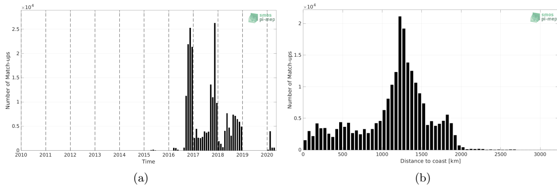
Figure 1: Number of match-ups between Surface drifters and SMAP SSS L2 v5.0 (JPL) SSS as a function of time (a) and as function of the distance to coast (b) over the Equatorial Ocean 10N-10S Pi-MEP region and for the full satellite product period.
