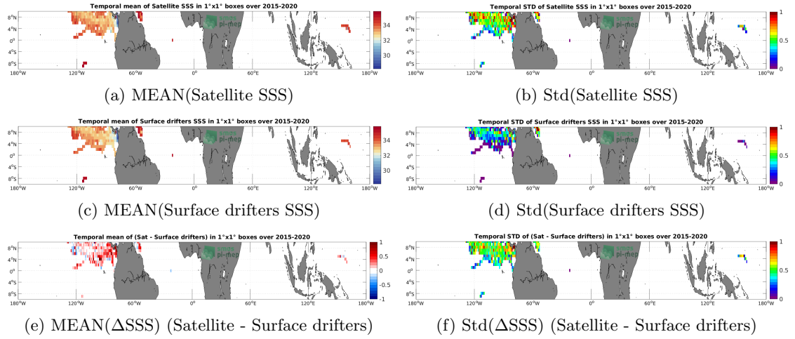
Figure 5: Temporal mean (left) and Std (right) of SSS from SMAP SSS L2 v5.0 (JPL) (top), Surface drifters (middle), and of \Delta SSS (Satellite - Surface drifters). Only match-up pairs are used to generate these maps.
