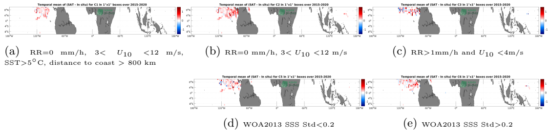
Figure 11: Temporal mean gridded over spatial boxes of size 1^\circ \times 1^\circ of \Delta SSS (SMAP SSS L2 v5.0 (JPL) - Surface drifters) for 5 different subdatasets corresponding to:RR=0 mm/h, 3 < U_{10} < 12 m/s, SST >5^\circ\text{C} , distance to coast > 800 km (a), RR=0 mm/h, 3 < U_{10} < 12 m/s (b), RR >1 mm/h and U_{10} < 4 m/s (c), WOA2013 SSS Std <0.2 (d), WOA2013 SSS Std >0.2 (e).
