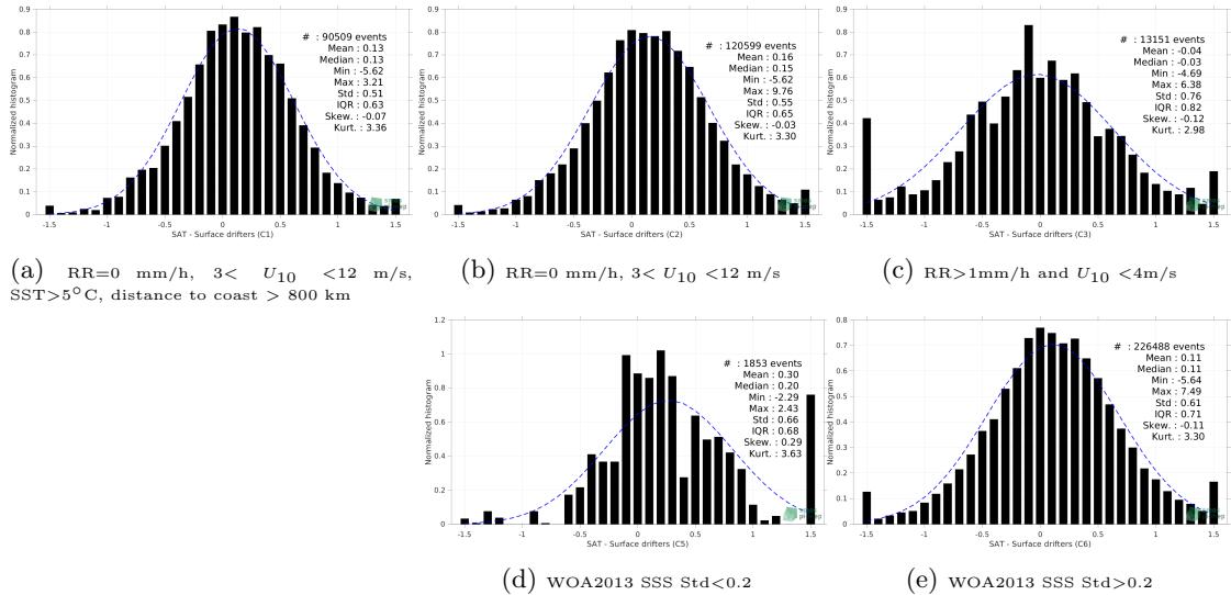
Figure 12: Normalized histogram of \Delta SSS (SMAP SSS L2 v5.0 (JPL) - Surface drifters) for 5 different subdatasets corresponding to: RR=0 mm/h, 3 < U_{10} < 12 m/s, SST >5^\circ\text{C} , distance to coast > 800 km (a), RR=0 mm/h, 3 < U_{10} < 12 m/s (b), RR >1 mm/h and U_{10} < 4 m/s (c), WOA2013 SSS Std <0.2 (d), WOA2013 SSS Std >0.2 (e).
