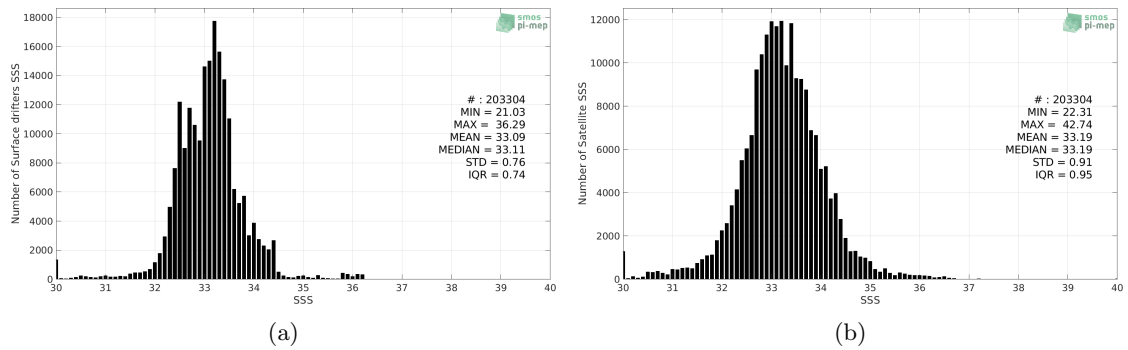
Figure 2: Histograms of SSS from Surface drifters (a) and SMAP SSS L2 v5.0 (JPL) (b) considering all match-up pairs per bins of 0.1 over the Equatorial Ocean 10N-10S Pi-MEP region and for the full satellite product period.
