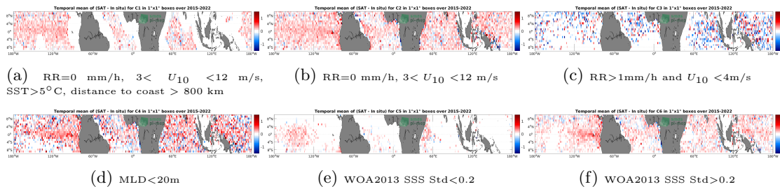
Figure 12: Temporal mean gridded over spatial boxes of size 1^\circ \times 1^\circ of \Delta SSS (SMAP SSS L2 v5.0 (JPL) - Argo) for 6 different subdatasets corresponding to:RR=0 mm/h, 3 < U_{10} < 12 m/s, SST>5°C, distance to coast > 800 km (a), RR=0 mm/h, 3 < U_{10} < 12 m/s (b), RR>1mm/h and U_{10} < 4 m/s (c),MLD<20m (d),WOA2013 SSS Std<0.2 (e),WOA2013 SSS Std>0.2 (f).
