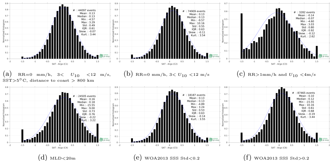
Figure 13: Normalized histogram of \Delta SSS (SMAP SSS L2 v5.0 (JPL) - Argo) for 6 different subdatasets corresponding to: RR=0 mm/h, 3 < U_{10} < 12 m/s, SST> 5^\circ C , distance to coast > 800 km (a), RR=0 mm/h, 3 < U_{10} < 12 m/s (b), RR>1mm/h and U_{10} < 4 m/s (c), MLD<20m (d), WOA2013 SSS Std<0.2 (e), WOA2013 SSS Std>0.2 (f).
