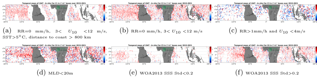
Figure 12: Temporal mean gridded over spatial boxes of size 1°x1° of \Delta SSS (SMAP SSS L2 v5.0 (JPL) - Argo) for 6 different subdatasets corresponding to:RR=0 mm/h, 3 < U_{10} < 12 m/s, SST>5°C, distance to coast > 800 km (a), RR=0 mm/h, 3 < U_{10} < 12 m/s (b), RR>1mm/h and U_{10} < 4m/s (c),MLD<20m (d),WOA2013 SSS Std<0.2 (e),WOA2013 SSS Std>0.2 (f).
