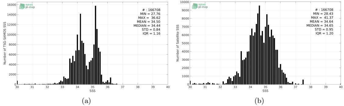
Figure 2: Histograms of SSS from TSG-SAMOS (a) and SMAP-L2-JPL-V4 (b) considering all match-up pairs per bins of 0.1 over the Equatorial Ocean 10N-10S Pi-MEP region and for the full satellite product period.
