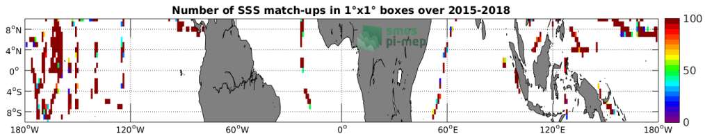
Figure 4: Number of SSS match-ups between TSG-SAMOS SSS and the SMAP-L2-JPL-V4 SSS product for the Equatorial Ocean 10N-10S Pi-MEP region over 1^\circ \times 1^\circ boxes and for the full satellite product period.
