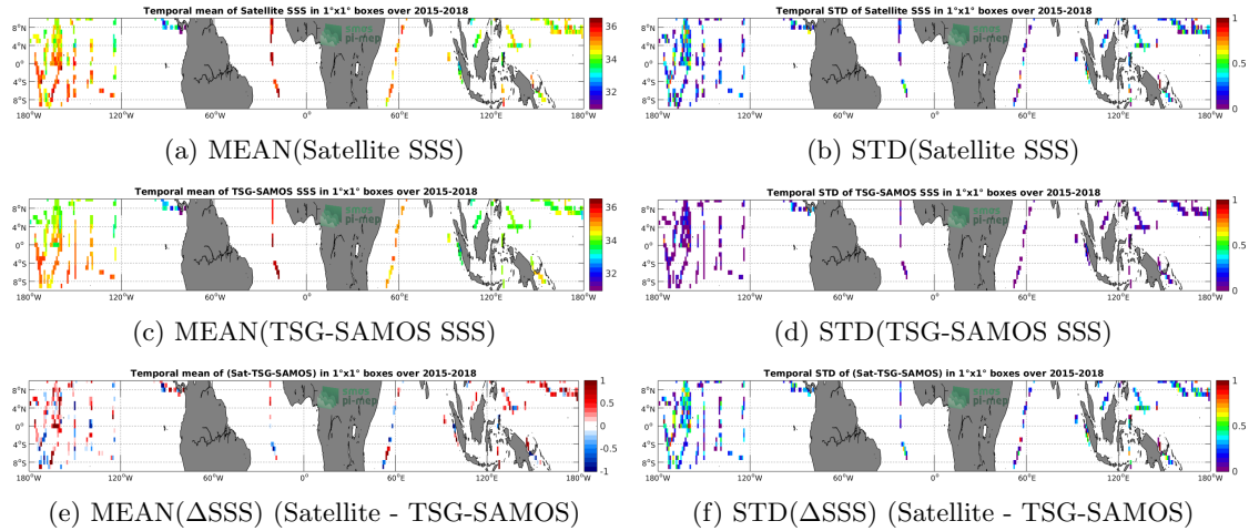
Figure 6: Temporal mean (left) and STD (right) of SSS from SMAP-L2-JPL-V4 (top), TSG-SAMOS (middle), and of \Delta SSS (Satellite - TSG-SAMOS). Only match-up pairs are used to generate these maps.
