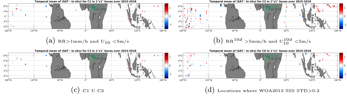
Figure 12: Temporal mean gridded over spatial boxes of size 1^\circ \times 1^\circ of \Delta SSS (SMAP-L2-JPL-V4 - TSG-SAMOS) for 4 different subdatasets corresponding to: RR > 1\text{mm/h} and U_{10} < 5\text{m/s} (a), RR^{10d} > 5\text{mm/h} and U_{10}^{10d} < 5\text{m/s} (b), C1 U C2 (c), Locations where WOA2013 SSS STD > 0.2 (d).
