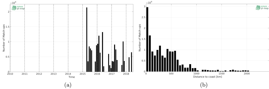
Figure 1: Number of match-ups between TSG-SAMOS and SMAP-L2-JPL-V4 SSS as a function of time (a) and as function of the distance to coast (b) over the Equatorial Ocean 10N-10S Pi-MEP region and for the full satellite product period.
