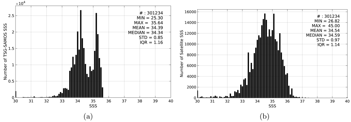
Figure 2: Histograms of SSS from TSG-SAMOS (a) and SMAP-L2-JPL-V4 (b) considering all match-up pairs per bins of 0.1 over the Equatorial Ocean 10N-10S Pi-MEP region and for the full satellite product period.
