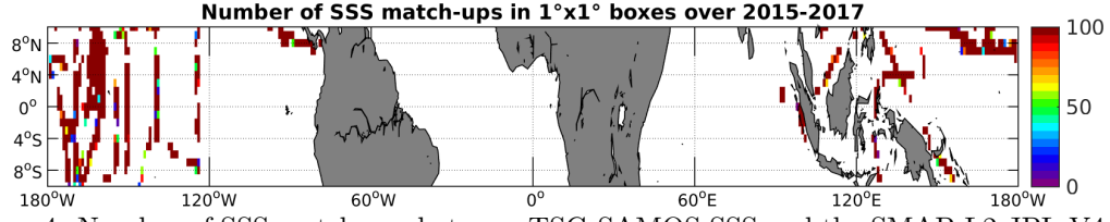
Figure 4: Number of SSS match-ups between TSG-SAMOS SSS and the SMAP-L2-JPL-V4 SSS product for the Equatorial Ocean 10N-10S Pi-MEP region over 1°x1° boxes and for the full satellite product period.
