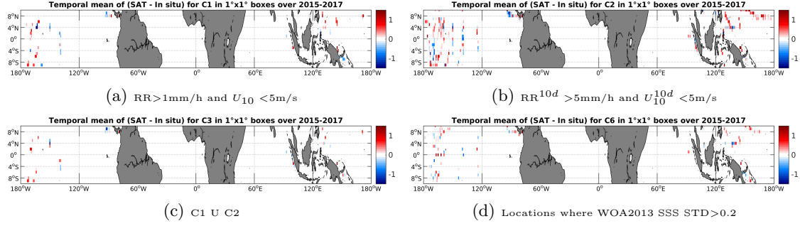
Figure 12: Temporal mean gridded over spatial boxes of size 1^\circ \times 1^\circ of \Delta SSS (SMAP-L2-JPL-V4 - TSG-SAMOS) for 4 different subdatasets corresponding to: RR > 1 mm/h and U_{10} < 5 m/s (a), RR ^{10d} > 5 mm/h and U_{10}^{10d} < 5 m/s (b), C1 U C2 (c), Locations where WOA2013 SSS STD > 0.2 (d).
