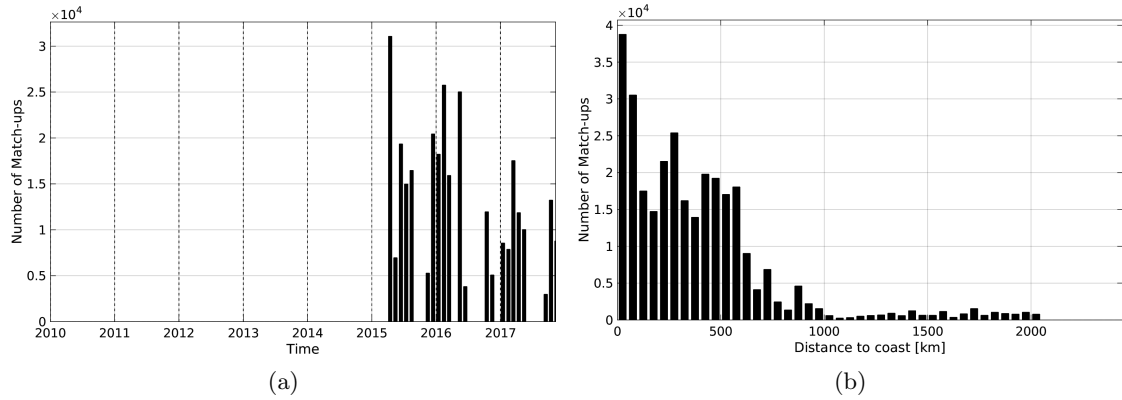
Figure 1: Number of match-ups between TSG-SAMOS and SMAP-L2-JPL-V4 SSS as a function of time (a) and as function of the distance to coast (b) over the Equatorial Ocean 10N-10S Pi-MEP region and for the full satellite product period.
