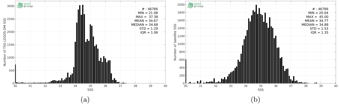
Figure 2: Histograms of SSS from TSG-LEGOS-DM (a) and SMAP-L2-JPL-V4 (b) considering all match-up pairs per bins of 0.1 over the Equatorial Ocean 10N-10S Pi-MEP region and for the full satellite product period.
