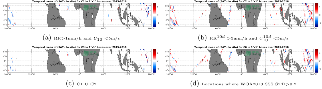
Figure 12: Temporal mean gridded over spatial boxes of size 1^\circ \times 1^\circ of \Delta SSS (SMAP-L2-JPL-V4 - TSG-LEGOS-DM) for 4 different subdatasets corresponding to: RR > 1\text{mm/h} and U_{10} < 5\text{m/s} (a), RR^{10d} > 5\text{mm/h} and U_{10}^{10d} < 5\text{m/s} (b), C1 U C2 (c), Locations where WOA2013 SSS STD > 0.2 (d).
