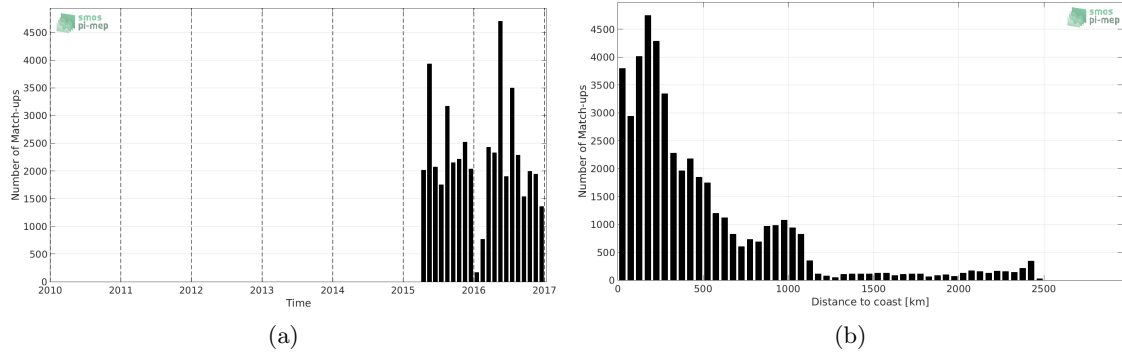
Figure 1: Number of match-ups between TSG-LEGOS-DM and SMAP-L2-JPL-V4 SSS as a function of time (a) and as function of the distance to coast (b) over the Equatorial Ocean 10N-10S Pi-MEP region and for the full satellite product period.
