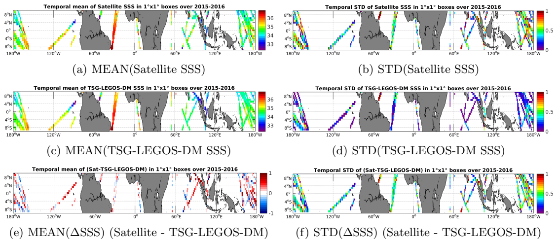
Figure 6: Temporal mean (left) and STD (right) of SSS from SMAP-L2-JPL-V4 (top), TSG-LEGOS-DM (middle), and of \Delta SSS (Satellite - TSG-LEGOS-DM). Only match-up pairs are used to generate these maps.
