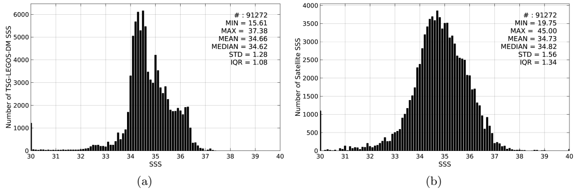
Figure 2: Histograms of SSS from TSG-LEGOS-DM (a) and SMAP-L2-JPL-V4 (b) considering all match-up pairs per bins of 0.1 over the Equatorial Ocean 10N-10S Pi-MEP region and for the full satellite product period.
