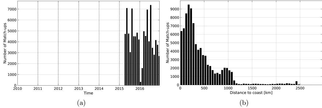
Figure 1: Number of match-ups between TSG-LEGOS-DM and SMAP-L2-JPL-V4 SSS as a function of time (a) and as function of the distance to coast (b) over the Equatorial Ocean 10N-10S Pi-MEP region and for the full satellite product period.
