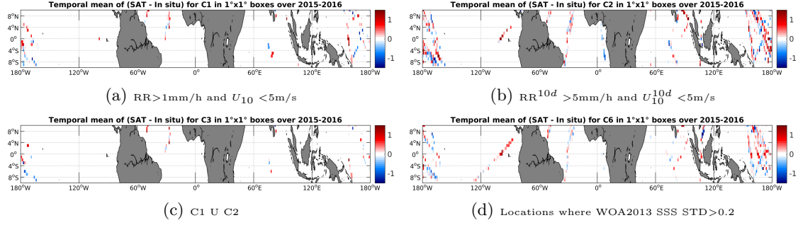
Figure 12: Temporal mean gridded over spatial boxes of size 1^\circ \times 1^\circ of \Delta SSS (SMAP-L2-JPL-V4 - TSG-LEGOS-DM) for 4 different subdatasets corresponding to: RR > 1\text{mm/h} and U_{10} < 5\text{m/s} (a), RR^{10d} > 5\text{mm/h} and U_{10}^{10d} < 5\text{m/s} (b), C1 U C2 (c), Locations where WOA2013 SSS STD > 0.2 (d).
