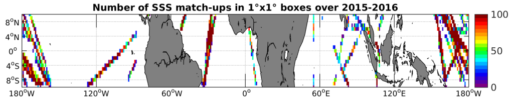
Figure 4: Number of SSS match-ups between TSG-LEGOS-DM SSS and the SMAP-L2-JPL-V4 SSS product for the Equatorial Ocean 10N-10S Pi-MEP region over 1^\circ \times 1^\circ boxes and for the full satellite product period.
