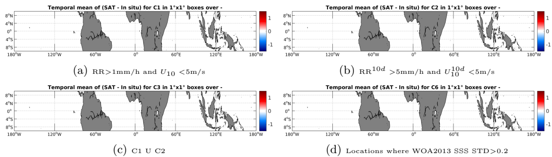
Figure 12: Temporal mean gridded over spatial boxes of size 1^\circ \times 1^\circ of \Delta SSS (SMAP-L2-JPL-V4 - TSG-GOSUD-Sailing-ship) for 4 different subdatasets corresponding to:RR > 1 mm/h and U_{10} < 5 m/s (a), RR ^{10d} > 5 mm/h and U_{10}^{10d} < 5 m/s (b), C1 U C2 (c),Locations where WOA2013 SSS STD > 0.2 (d).
