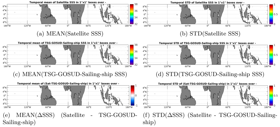
Figure 6: Temporal mean (left) and STD (right) of SSS from SMAP-L2-JPL-V4 (top), TSG-GOSUD-Sailing-ship (middle), and of \Delta SSS (Satellite - TSG-GOSUD-Sailing-ship). Only match-up pairs are used to generate these maps.
