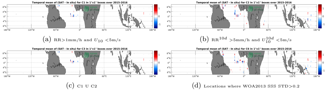
Figure 12: Temporal mean gridded over spatial boxes of size 1^\circ \times 1^\circ of \Delta SSS (SMAP-L2-JPL-V4 - TSG-GOSUD-Research-vessel) for 4 different subdatasets corresponding to: RR >1 mm/h and U_{10} < 5 m/s (a), RR ^{10d} > 5 mm/h and U_{10}^{10d} < 5 m/s (b), C1 U C2 (c), Locations where WOA2013 SSS STD >0.2 (d).
