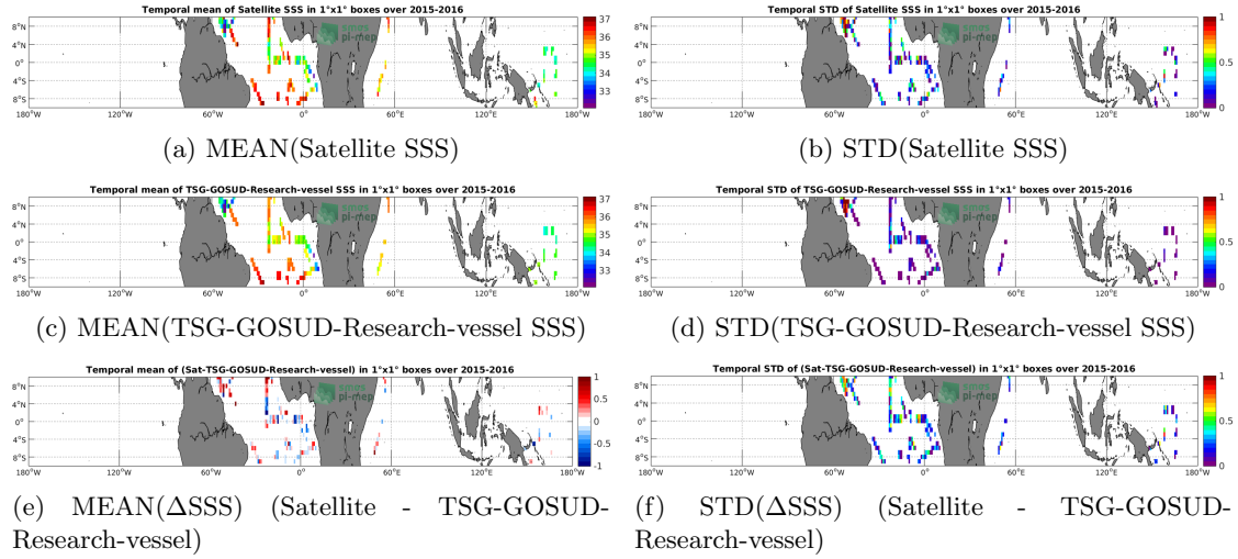
Figure 6: Temporal mean (left) and STD (right) of SSS from SMAP-L2-JPL-V4 (top), TSG-GOSUD-Research-vessel (middle), and of \Delta SSS (Satellite - TSG-GOSUD-Research-vessel). Only match-up pairs are used to generate these maps.
