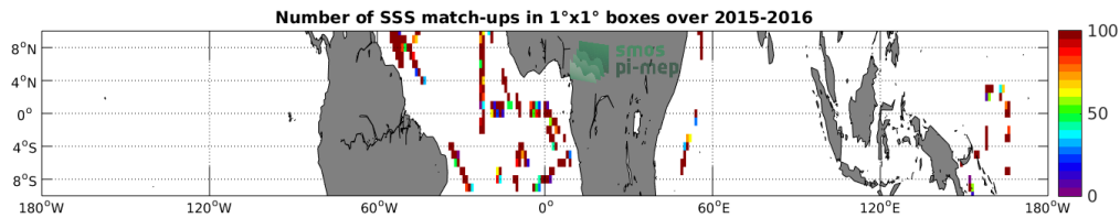
Figure 4: Number of SSS match-ups between TSG-GOSUD-Research-vessel SSS and the SMAP-L2-JPL-V4 SSS product for the Equatorial Ocean 10N-10S Pi-MEP region over 1^\circ \times 1^\circ boxes and for the full satellite product period.
