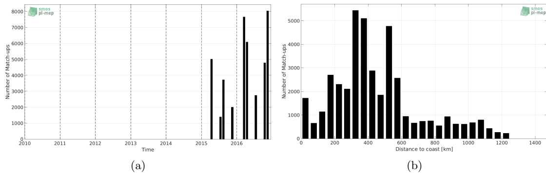
Figure 1: Number of match-ups between TSG-GOSUD-Research-vessel and SMAP-L2-JPL-V4 SSS as a function of time (a) and as function of the distance to coast (b) over the Equatorial Ocean 10N-10S Pi-MEP region and for the full satellite product period.
