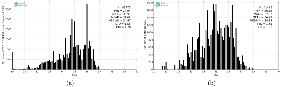
Figure 2: Histograms of SSS from TSG-GOSUD-Research-vessel (a) and SMAP-L2-JPL-V4 (b) considering all match-up pairs per bins of 0.1 over the Equatorial Ocean 10N-10S Pi-MEP region and for the full satellite product period.
