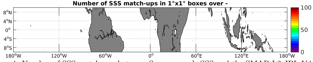
Figure 4: Number of SSS match-ups between Sea mammals SSS and the SMAP-L2-JPL-V4 SSS product for the Equatorial Ocean 10N-10S Pi-MEP region over 1^\circ \times 1^\circ boxes and for the full satellite product period.
