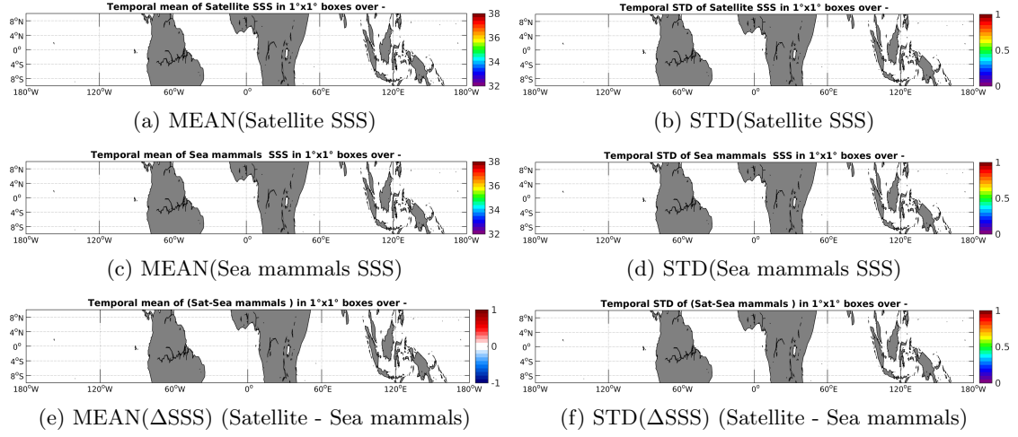
Figure 6: Temporal mean (left) and STD (right) of SSS from SMAP-L2-JPL-V4 (top), Sea mammals (middle), and of \Delta SSS (Satellite - Sea mammals). Only match-up pairs are used to generate these maps.
