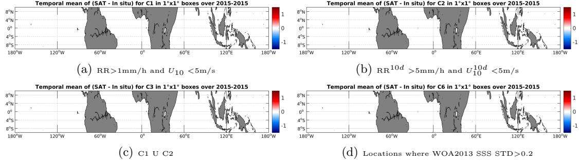
Figure 11: Temporal mean gridded over spatial boxes of size 1^\circ \times 1^\circ of \Delta SSS (SMAP-L2-JPL-V4 - Surface drifters) for 4 different subdatasets corresponding to: RR > 1 mm/h and U_{10} < 5 m/s (a), RR ^{10d} > 5 mm/h and U_{10}^{10d} < 5 m/s (b), C1 U C2 (c), Locations where WOA2013 SSS STD > 0.2 (d).
