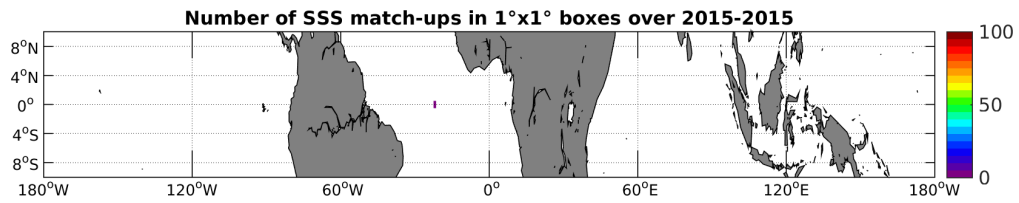
Figure 3: Number of SSS match-ups between Surface drifters SSS and the SMAP-L2-JPL-V4 SSS product for the Equatorial Ocean 10N-10S Pi-MEP region over 1°x1° boxes and for the full satellite product period.
