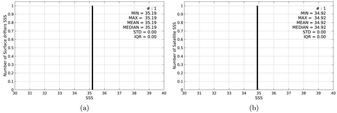
Figure 2: Histograms of SSS from Surface drifters (a) and SMAP-L2-JPL-V4 (b) considering all match-up pairs per bins of 0.1 over the Equatorial Ocean 10N-10S Pi-MEP region and for the full satellite product period.
