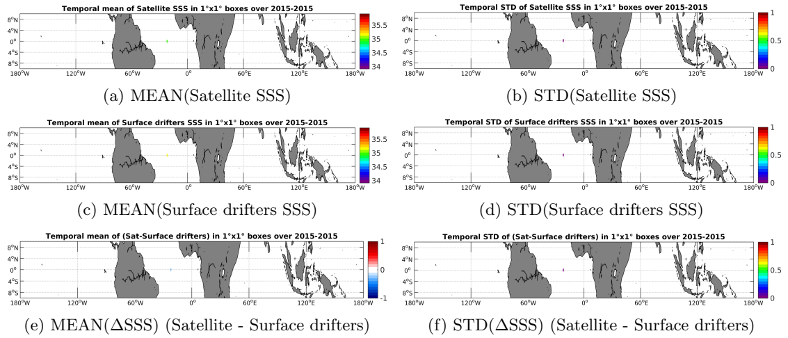
Figure 5: Temporal mean (left) and STD (right) of SSS from SMAP-L2-JPL-V4 (top), Surface drifters (middle), and of \Delta SSS (Satellite - Surface drifters). Only match-up pairs are used to generate these maps.
