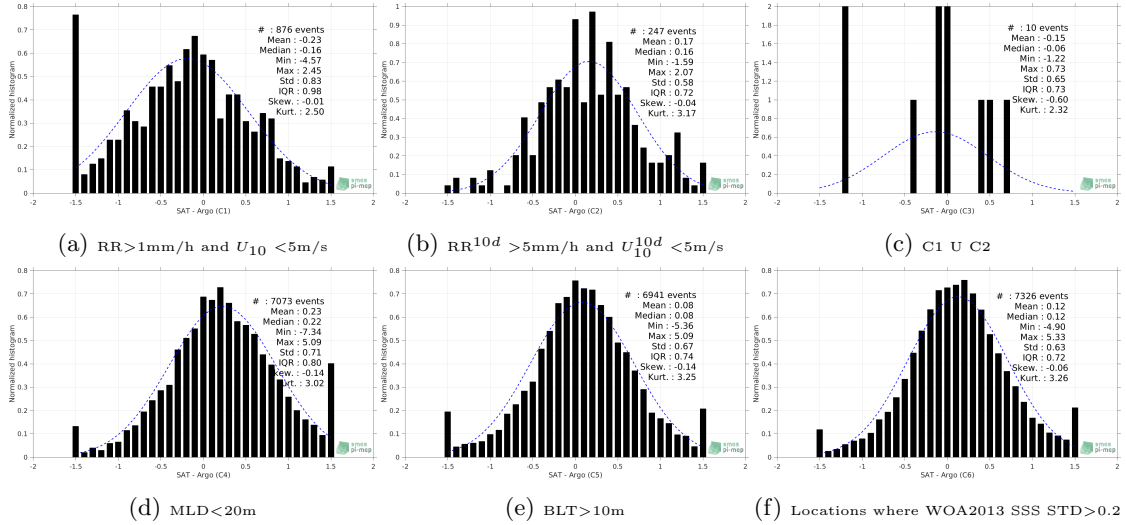
Figure 13: Normalized histogram of \Delta\text{SSS} (SMAP-L2-JPL-V4 - Argo) for 6 different subdatasets corresponding to: \text{RR} > 1\text{mm/h} and U_{10} < 5\text{m/s} (a), \text{RR}^{10d} > 5\text{mm/h} and U_{10}^{10d} < 5\text{m/s} (b), C1 U C2 (c), \text{MLD} < 20\text{m} (d), \text{BLT} > 10\text{m} (e), Locations where WOA2013 SSS \text{STD} > 0.2 (f).
