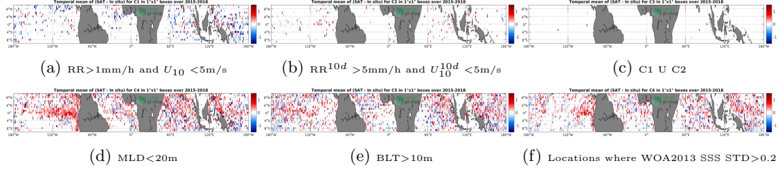
Figure 12: Temporal mean gridded over spatial boxes of size 1^\circ \times 1^\circ of \Delta\text{SSS} (SMAP-L2-JPL-V4 - Argo) for 6 different subdatasets corresponding to: \text{RR} > 1\text{mm/h} and U_{10} < 5\text{m/s} (a), \text{RR}^{10d} > 5\text{mm/h} and U_{10}^{10d} < 5\text{m/s} (b), C1 U C2 (c), \text{MLD} < 20\text{m} (d), \text{BLT} > 10\text{m} (e), Locations where WOA2013 SSS \text{STD} > 0.2 (f).
