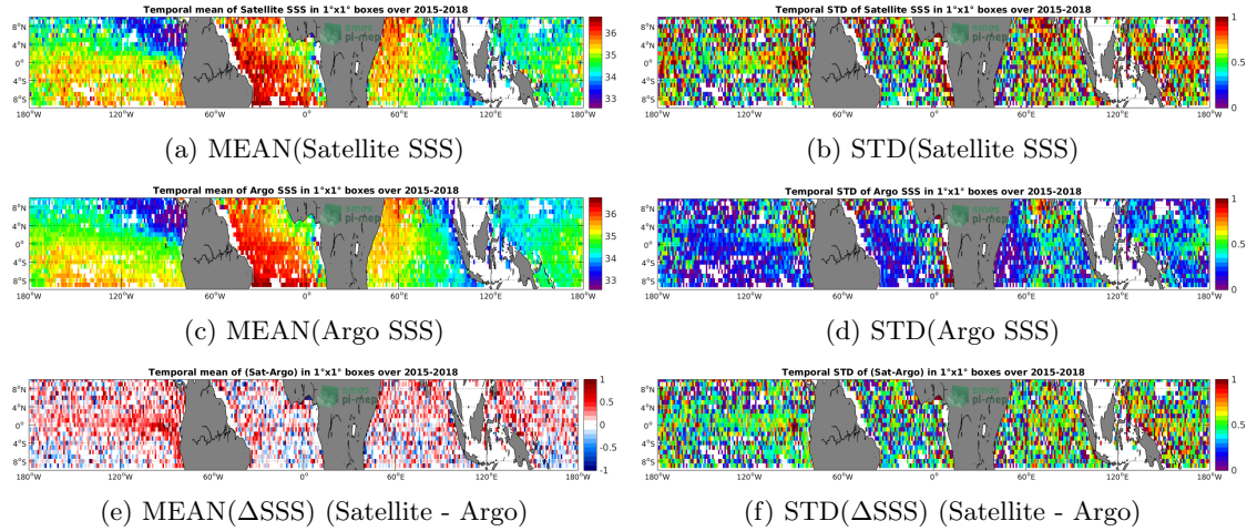
Figure 6: Temporal mean (left) and STD (right) of SSS from SMAP-L2-JPL-V4 (top), Argo (middle), and of \Delta SSS (Satellite - Argo). Only match-up pairs are used to generate these maps.
