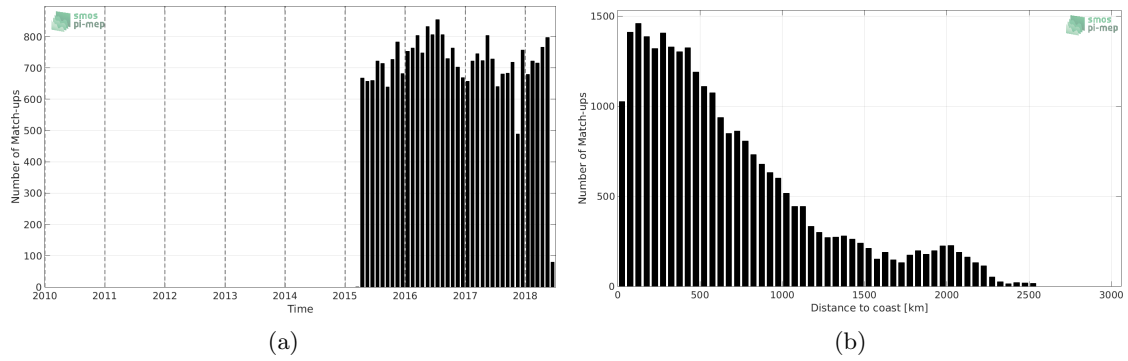
Figure 1: Number of match-ups between Argo and SMAP-L2-JPL-V4 SSS as a function of time (a) and as function of the distance to coast (b) over the Equatorial Ocean 10N-10S Pi-MEP region and for the full satellite product period.
