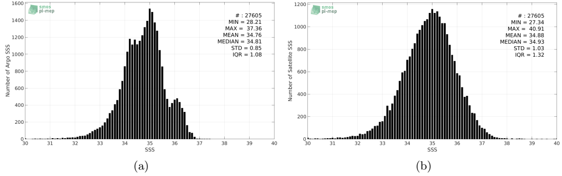
Figure 2: Histograms of SSS from Argo (a) and SMAP-L2-JPL-V4 (b) considering all match-up pairs per bins of 0.1 over the Equatorial Ocean 10N-10S Pi-MEP region and for the full satellite product period.
