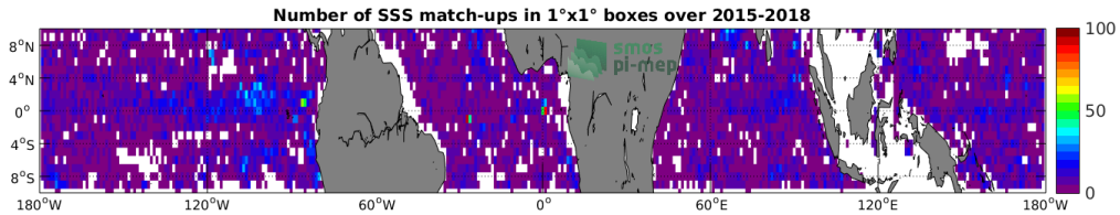
Figure 4: Number of SSS match-ups between Argo SSS and the SMAP-L2-JPL-V4 SSS product for the Equatorial Ocean 10N-10S Pi-MEP region over 1°x1° boxes and for the full satellite product period.
