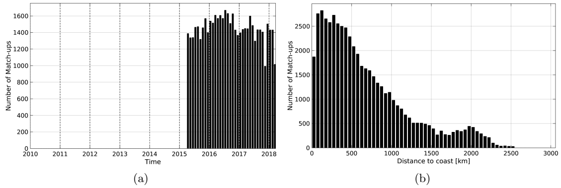
Figure 1: Number of match-ups between Argo and SMAP-L2-JPL-V4 SSS as a function of time (a) and as function of the distance to coast (b) over the Equatorial Ocean 10N-10S Pi-MEP region and for the full satellite product period.
