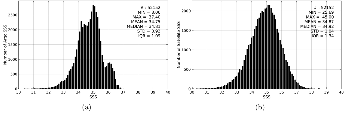
Figure 2: Histograms of SSS from Argo (a) and SMAP-L2-JPL-V4 (b) considering all match-up pairs per bins of 0.1 over the Equatorial Ocean 10N-10S Pi-MEP region and for the full satellite product period.
