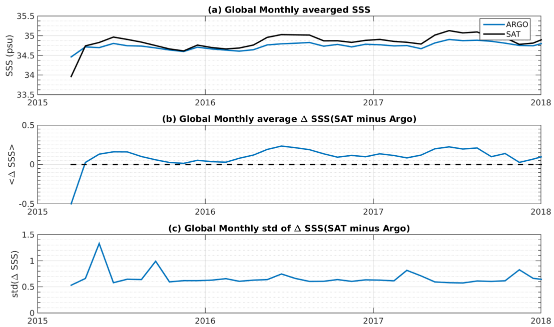
Figure 7: Time series of the monthly averaged mean SSS (top), mean \Delta SSS (Satellite - Argo) and STD of \Delta SSS (Satellite - Argo) over the Equatorial Ocean 10N-10S Pi-MEP region considering all match-ups collected by the Pi-MEP platform.
