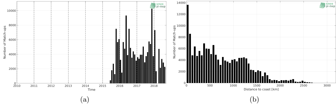
Figure 1: Number of match-ups between TSG-LEGOS-DM and SMAP-L2-JPL-V4.2 SSS as a function of time (a) and as function of the distance to coast (b) over the Equatorial Ocean 10N-10S Pi-MEP region and for the full satellite product period.
