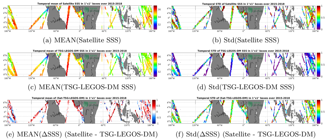
Figure 6: Temporal mean (left) and Std (right) of SSS from SMAP-L2-JPL-V4.2 (top), TSG-LEGOS-DM (middle), and of \Delta SSS (Satellite - TSG-LEGOS-DM). Only match-up pairs are used to generate these maps.
