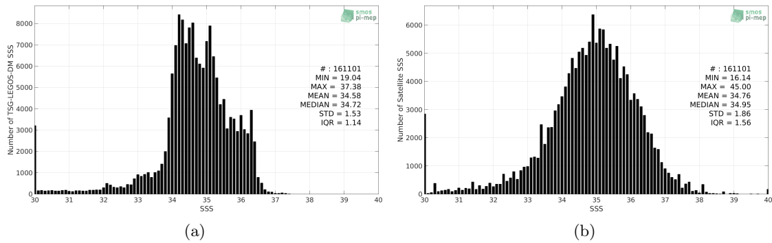
Figure 2: Histograms of SSS from TSG-LEGOS-DM (a) and SMAP-L2-JPL-V4.2 (b) considering all match-up pairs per bins of 0.1 over the Equatorial Ocean 10N-10S Pi-MEP region and for the full satellite product period.
