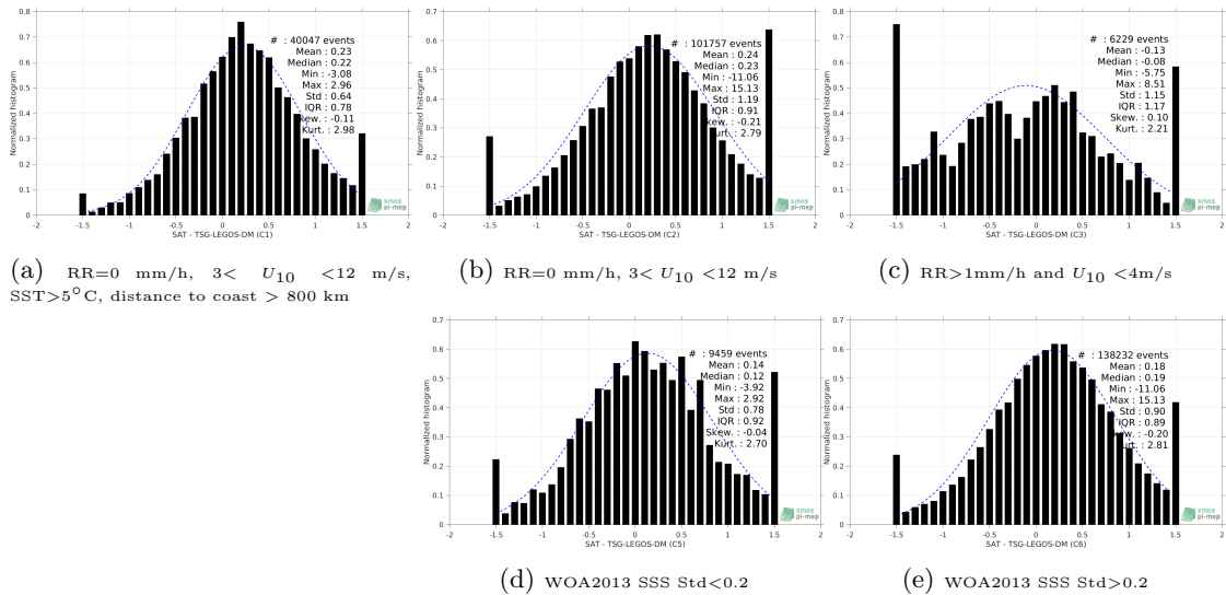
Figure 13: Normalized histogram of \Delta SSS (SMAP-L2-JPL-V4.2 - TSG-LEGOS-DM) for 5 different subdatasets corresponding to: RR=0 mm/h, 3 < U_{10} < 12 m/s, SST >5^\circ C , distance to coast > 800 km (a), RR=0 mm/h, 3 < U_{10} < 12 m/s (b), RR >1 mm/h and U_{10} < 4 m/s (c), WOA2013 SSS Std <0.2 (d), WOA2013 SSS Std >0.2 (e).
