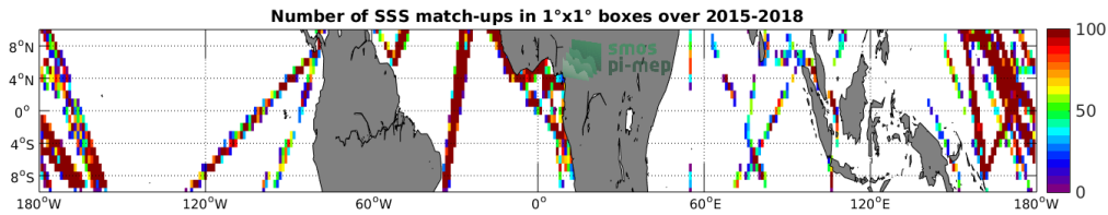
Figure 4: Number of SSS match-ups between TSG-LEGOS-DM SSS and the SMAP-L2-JPL-V4.2 SSS product for the Equatorial Ocean 10N-10S Pi-MEP region over 1^\circ \times 1^\circ boxes and for the full satellite product period.
