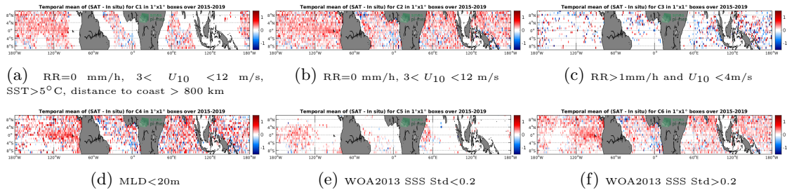
Figure 12: Temporal mean gridded over spatial boxes of size 1^\circ \times 1^\circ of \Delta SSS (SMAP-L2-JPL-V4.2 - Argo) for 6 different subdatasets corresponding to:RR=0 mm/h, 3 < U_{10} < 12 m/s, SST >5^\circ C, distance to coast > 800 km (a), RR=0 mm/h, 3 < U_{10} < 12 m/s (b), RR >1 mm/h and U_{10} < 4 m/s (c),MLD <20 m (d),WOA2013 SSS Std <0.2 (e),WOA2013 SSS Std >0.2 (f).
