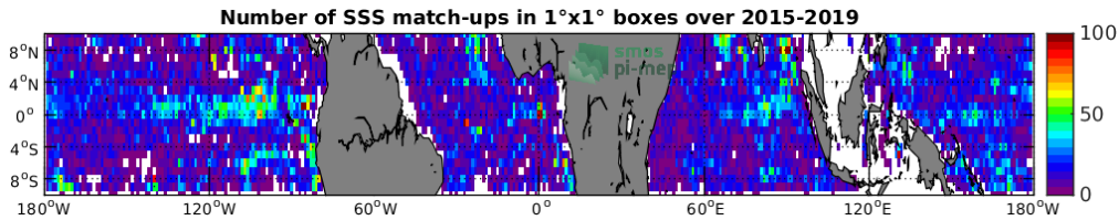
Figure 4: Number of SSS match-ups between Argo SSS and the SMAP-L2-JPL-V4.2 SSS product for the Equatorial Ocean 10N-10S Pi-MEP region over 1^\circ \times 1^\circ boxes and for the full satellite product period.
