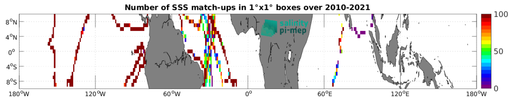
Figure 5: Number of SSS match-ups between TSG (GOSUD-Sailing-ship) SSS and the ISAS v7 - Monthly (Ifremer-LOPS-CMEMS) SSS product for the Equatorial Ocean 10N-10S Pi-MEP region over 1^\circ \times 1^\circ boxes and for the full satellite product period.
