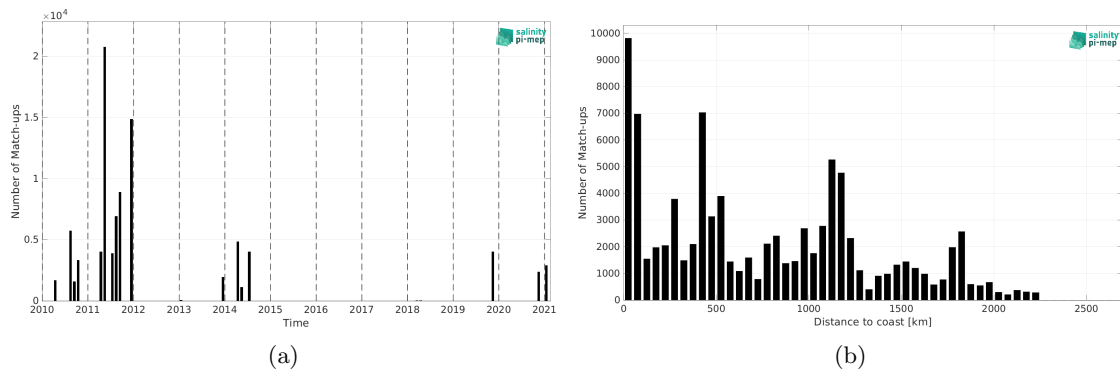
Figure 2: Number of match-ups between TSG (GOSUD-Sailing-ship) and ISAS v7 - Monthly (Ifremer-LOPS-CMEMS) SSS as a function of time (a) and as function of the distance to coast (b) over the Equatorial Ocean 10N-10S Pi-MEP region and for the full satellite product period.
