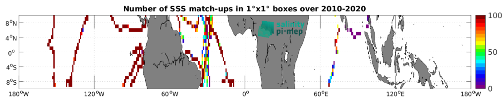
Figure 5: Number of SSS match-ups between TSG (GOSUD-Sailing-ship) SSS and the ISAS SSS product for the Equatorial Ocean 10N-10S Pi-MEP region over 1^\circ \times 1^\circ boxes and for the full satellite product period.
