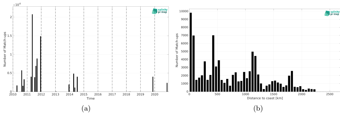
Figure 2: Number of match-ups between TSG (GOSUD-Sailing-ship) and ISAS SSS as a function of time (a) and as function of the distance to coast (b) over the Equatorial Ocean 10N-10S Pi-MEP region and for the full satellite product period.
