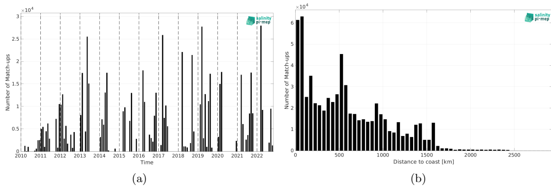
Figure 2: Number of match-ups between TSG (GOSUD-Research-vessel) and ISAS v7 - Monthly (Ifremer-LOPS-CMEMS) SSS as a function of time (a) and as function of the distance to coast (b) over the Equatorial Ocean 10N-10S Pi-MEP region and for the full satellite product period.
