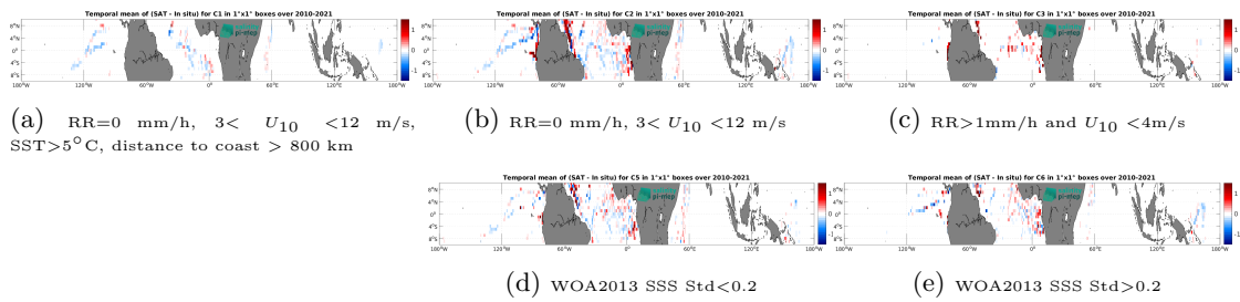
Figure 14: Temporal mean gridded over spatial boxes of size 1^\circ \times 1^\circ of \Delta SSS (ISAS - TSG (GOSUD-Research-vessel)) for 5 different subdatasets corresponding to:RR=0 mm/h, 3 < U_{10} < 12 m/s, SST>5°C, distance to coast > 800 km (a), RR=0 mm/h, 3 < U_{10} < 12 m/s (b), RR>1mm/h and U_{10} < 4 m/s (c), WOA2013 SSS Std<0.2 (d), WOA2013 SSS Std>0.2 (e).
