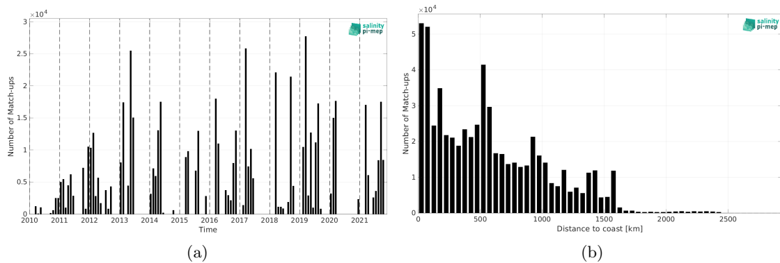
Figure 2: Number of match-ups between TSG (GOSUD-Research-vessel) and ISAS SSS as a function of time (a) and as function of the distance to coast (b) over the Equatorial Ocean 10N-10S Pi-MEP region and for the full satellite product period.
