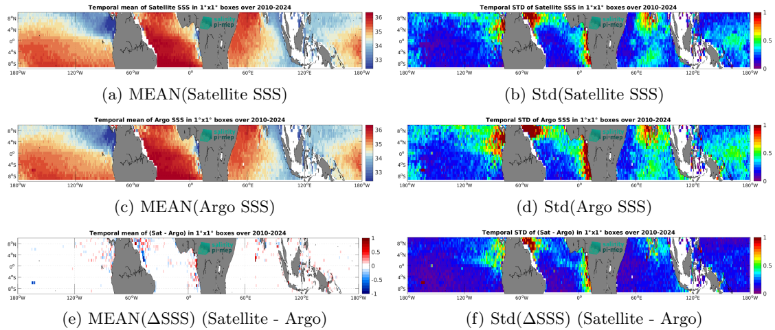
Figure 7: Temporal mean (left) and Std (right) of SSS from ISAS v7 - Monthly (Ifremer-LOPS-CMEMS) (top), Argo (middle), and of \Delta SSS (Satellite - Argo). Only match-up pairs are used to generate these maps.
