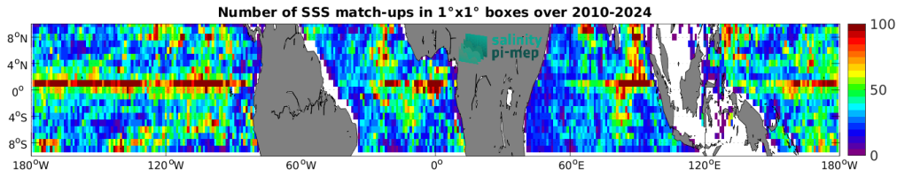
Figure 5: Number of SSS match-ups between Argo SSS and the ISAS v7 - Monthly (Ifremer-LOPS-CMEMS) SSS product for the Equatorial Ocean 10N-10S Pi-MEP region over 1^\circ \times 1^\circ boxes and for the full satellite product period.
