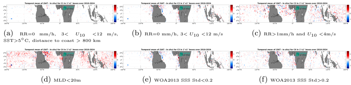
Figure 14: Temporal mean gridded over spatial boxes of size 1^\circ \times 1^\circ of \Delta SSS (ISAS v7 - Monthly (Ifremer-LOPS-CMEMS) - Argo) for 6 different subdatasets corresponding to:RR=0 mm/h, 3 < U_{10} < 12 m/s, SST >5^\circ\text{C} , distance to coast > 800 km (a), RR=0 mm/h, 3 < U_{10} < 12 m/s (b), RR >1 mm/h and U_{10} < 4 m/s (c),MLD <20 m (d),WOA2013 SSS Std <0.2 (e),WOA2013 SSS Std >0.2 (f).
