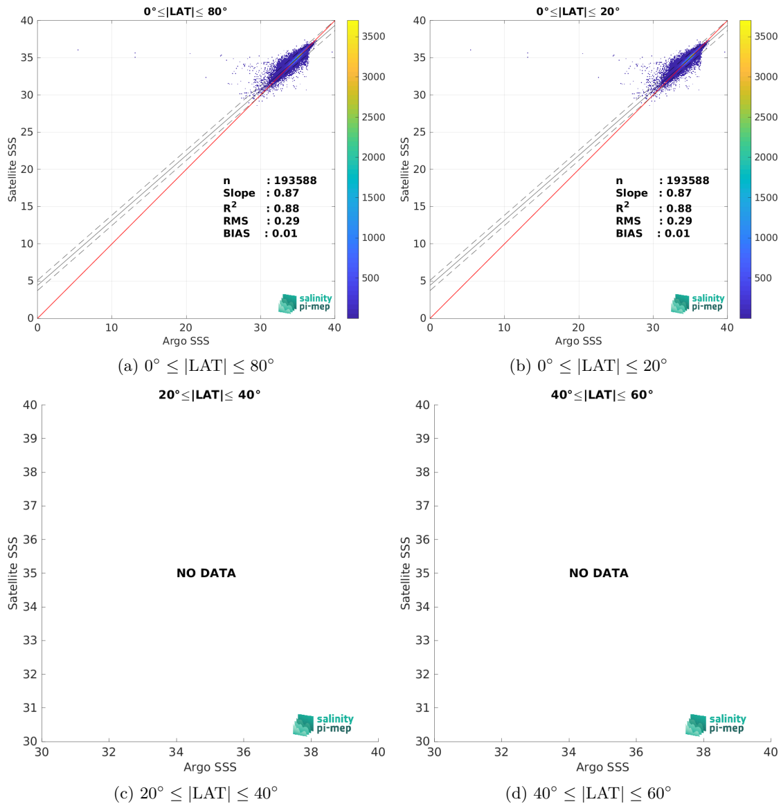
Figure 10: Contour maps of the concentration of ISAS v7 - Monthly (Ifremer-LOPS-CMEMS) SSS (y-axis) versus Argo SSS (x-axis) at match-up pairs for different latitude bands. For each plot, the red line shows x=y . The black thin and dashed lines indicate a linear fit through the data cloud and the \pm 95\% confidence levels, respectively. The number match-up pairs n , the slope and R^2 coefficient of the linear fit, the root mean square (RMS) and the mean bias between satellite and in situ data are indicated for each latitude band in each plots.
