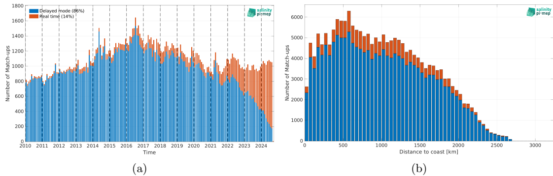
Figure 2: Number of match-ups between Argo and ISAS v7 - Monthly (Ifremer-LOPS-CMEMS) SSS as a function of time (a) and as function of the distance to coast (b) over the Equatorial Ocean 10N-10S Pi-MEP region and for the full satellite product period.
