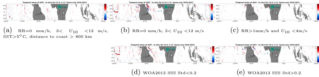
Figure 14: Temporal mean gridded over spatial boxes of size 1^\circ \times 1^\circ of \Delta SSS (CCI SSS L4 Merged-OI v5.5 - 7-day running (ESA) - TSG (SAMOS)) for 5 different subdatasets corresponding to:RR=0 mm/h, 3 < U_{10} < 12 m/s, SST >5^\circ\text{C} , distance to coast > 800 km (a), RR=0 mm/h, 3 < U_{10} < 12 m/s (b), RR >1 mm/h and U_{10} < 4 m/s (c), WOA2013 SSS Std <0.2 (d), WOA2013 SSS Std >0.2 (e).
