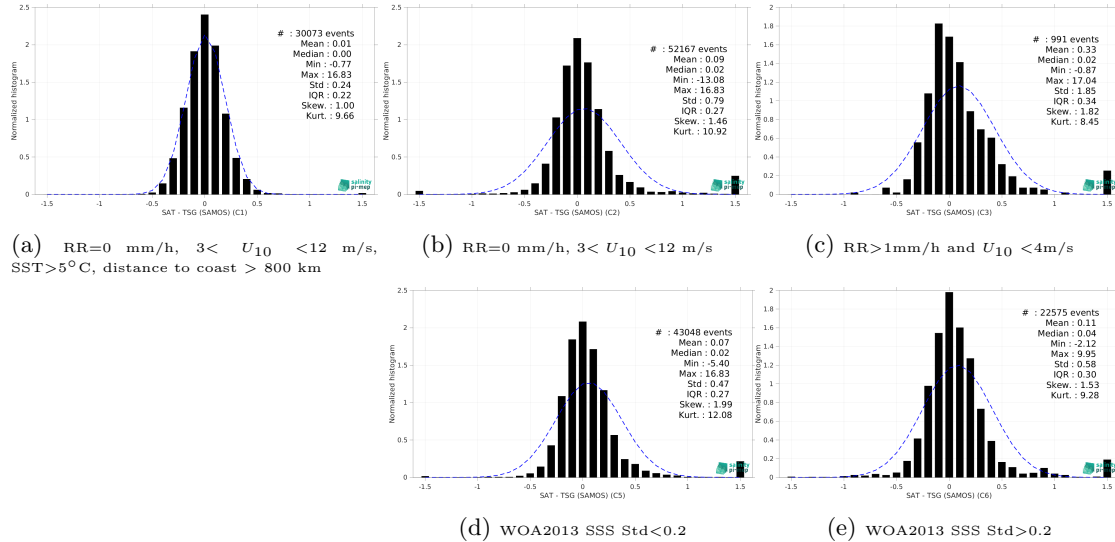
Figure 15: Normalized histogram of \Delta SSS (CCI SSS L4 Merged-OI v5.5 - 7-day running (ESA) - TSG (SAMOS)) for 5 different subdatasets corresponding to: RR=0 mm/h, 3 < U_{10} < 12 m/s, SST >5^\circ\text{C} , distance to coast > 800 km (a), RR=0 mm/h, 3 < U_{10} < 12 m/s (b), RR >1 mm/h and U_{10} < 4 m/s (c), WOA2013 SSS Std <0.2 (d), WOA2013 SSS Std >0.2 (e).
