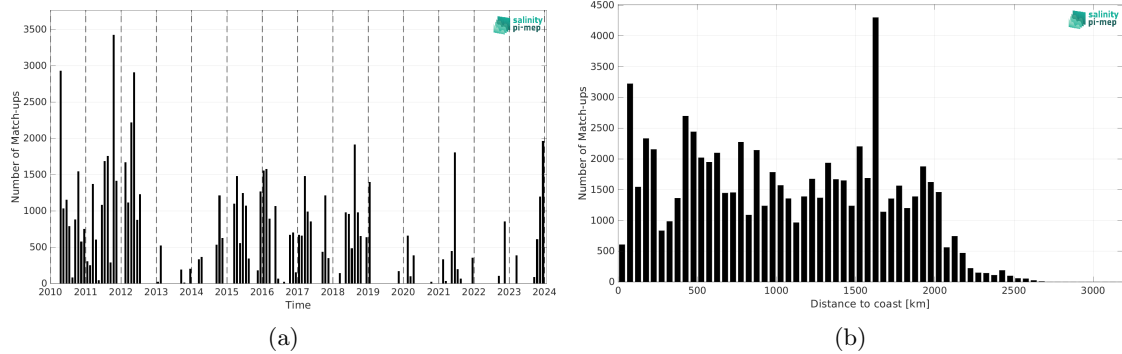
Figure 2: Number of match-ups between TSG (SAMOS) and CCI SSS L4 Merged-OI v5.5 - 7-day running (ESA) SSS as a function of time (a) and as function of the distance to coast (b) over the Equatorial Ocean 10N-10S Pi-MEP region and for the full satellite product period.
