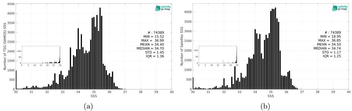
Figure 3: Histograms of SSS from TSG (SAMOS) (a) and CCI SSS L4 Merged-OI v5.5 - 7-day running (ESA) (b) considering all match-up pairs per bins of 0.1 over the Equatorial Ocean 10N-10S Pi-MEP region and for the full satellite product period.
