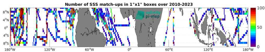
Figure 5: Number of SSS match-ups between TSG (SAMOS) SSS and the CCI SSS L4 Merged-OI v5.5 - 7-day running (ESA) SSS product for the Equatorial Ocean 10N-10S Pi-MEP region over 1^\circ \times 1^\circ boxes and for the full satellite product period.
