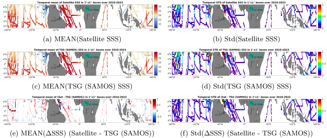
Figure 7: Temporal mean (left) and Std (right) of SSS from CCI SSS L4 Merged-OI v5.5 - 7-day running (ESA) (top), TSG (SAMOS) (middle), and of \Delta SSS (Satellite - TSG (SAMOS)). Only match-up pairs are used to generate these maps.
