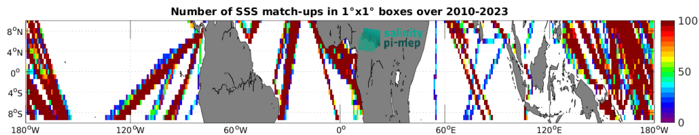
Figure 5: Number of SSS match-ups between TSG (LEGOS-DM) SSS and the CCI SSS L4 Merged-OI v5.5 - 7-day running (ESA) SSS product for the Equatorial Ocean 10N-10S Pi-MEP region over 1^\circ \times 1^\circ boxes and for the full satellite product period.
