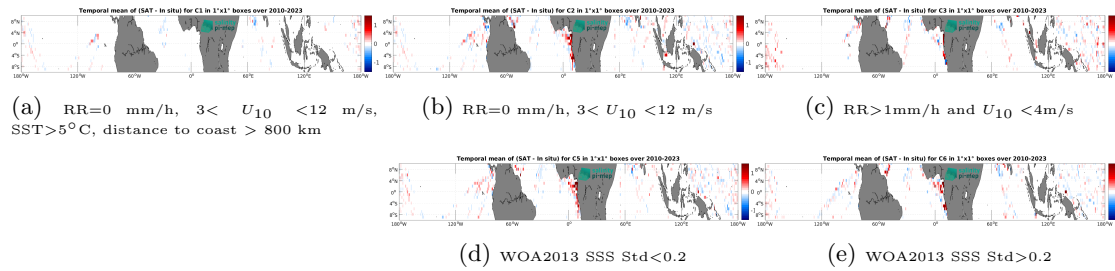
Figure 14: Temporal mean gridded over spatial boxes of size 1^\circ \times 1^\circ of \Delta\text{SSS} (CCI SSS L4 Merged-OI v5.5 - 7-day running (ESA) - TSG (LEGOS-DM)) for 5 different subdatasets corresponding to: RR=0 mm/h, 3 < U_{10} < 12 m/s, SST>5°C, distance to coast > 800 km (a), RR=0 mm/h, 3 < U_{10} < 12 m/s (b), RR>1mm/h and U_{10} < 4 m/s (c), WOA2013 SSS Std<0.2 (d), WOA2013 SSS Std>0.2 (e).
