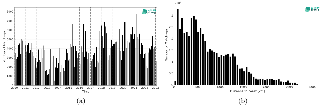
Figure 2: Number of match-ups between TSG (LEGOS-DM) and CCI SSS L4 Merged-OI v5.5 - 7-day running (ESA) SSS as a function of time (a) and as function of the distance to coast (b) over the Equatorial Ocean 10N-10S Pi-MEP region and for the full satellite product period.
