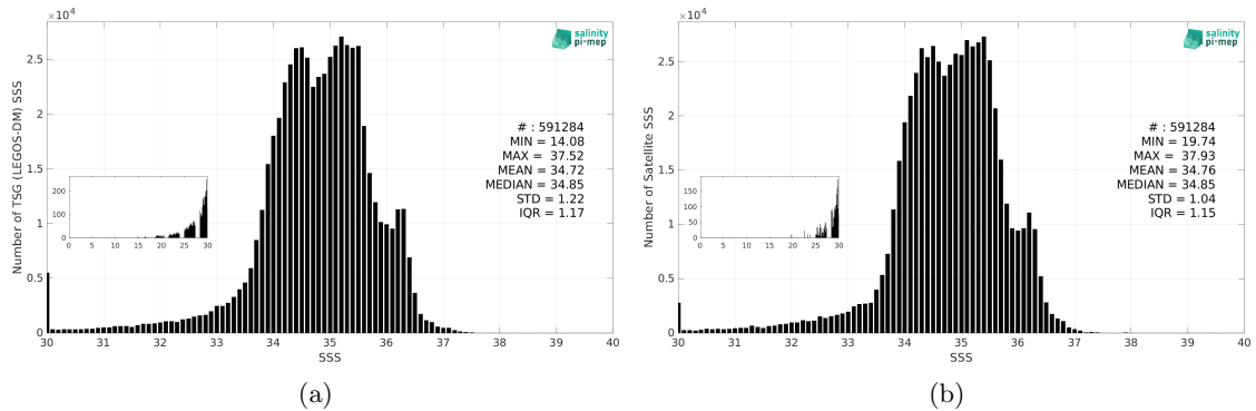
Figure 3: Histograms of SSS from TSG (LEGOS-DM) (a) and CCI SSS L4 Merged-OI v5.5 - 7-day running (ESA) (b) considering all match-up pairs per bins of 0.1 over the Equatorial Ocean 10N-10S Pi-MEP region and for the full satellite product period.
