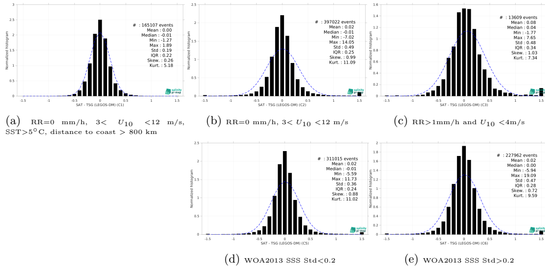
Figure 15: Normalized histogram of \Delta\text{SSS} (CCI SSS L4 Merged-OI v5.5 - 7-day running (ESA) - TSG (LEGOS-DM)) for 5 different subdatasets corresponding to: RR=0 mm/h, 3 < U_{10} < 12 m/s, SST>5°C, distance to coast > 800 km (a), RR=0 mm/h, 3 < U_{10} < 12 m/s (b), RR>1mm/h and U_{10} < 4 m/s (c), WOA2013 SSS Std<0.2 (d), WOA2013 SSS Std>0.2 (e).
