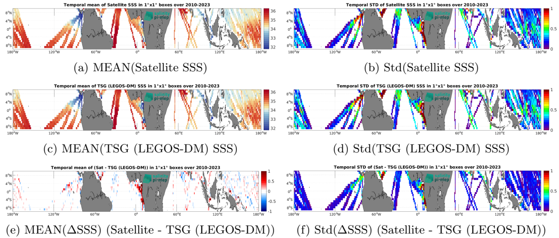
Figure 7: Temporal mean (left) and Std (right) of SSS from CCI SSS L4 Merged-OI v5.5 - 7-day running (ESA) (top), TSG (LEGOS-DM) (middle), and of \Delta SSS (Satellite - TSG (LEGOS-DM)). Only match-up pairs are used to generate these maps.
